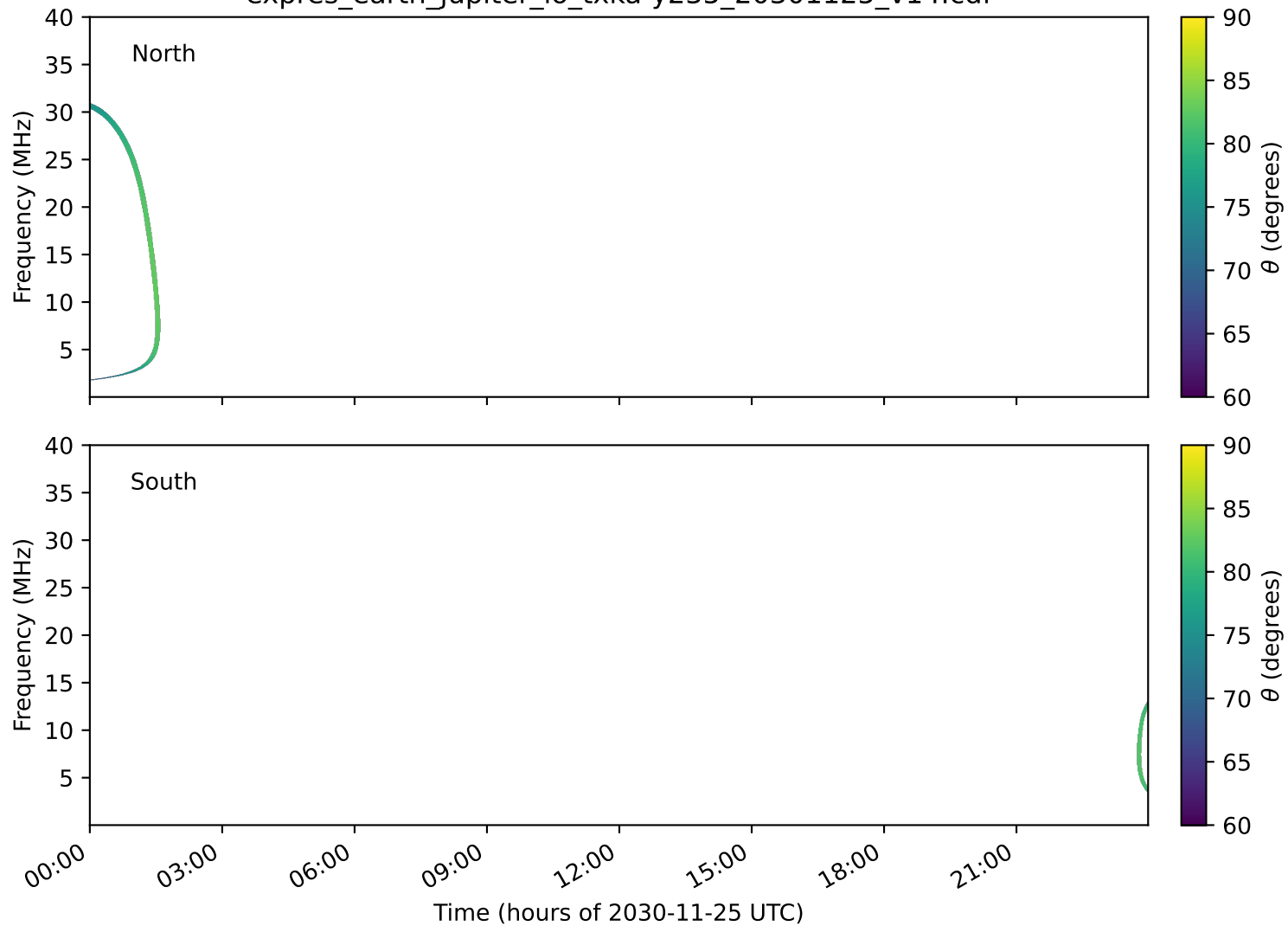
expres_earth_jupiter_io_txka-y235_20301125_v14.cdf
