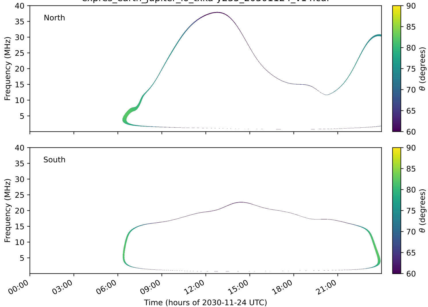
expres_earth_jupiter_io_txka-y235_20301124_v14.cdf
