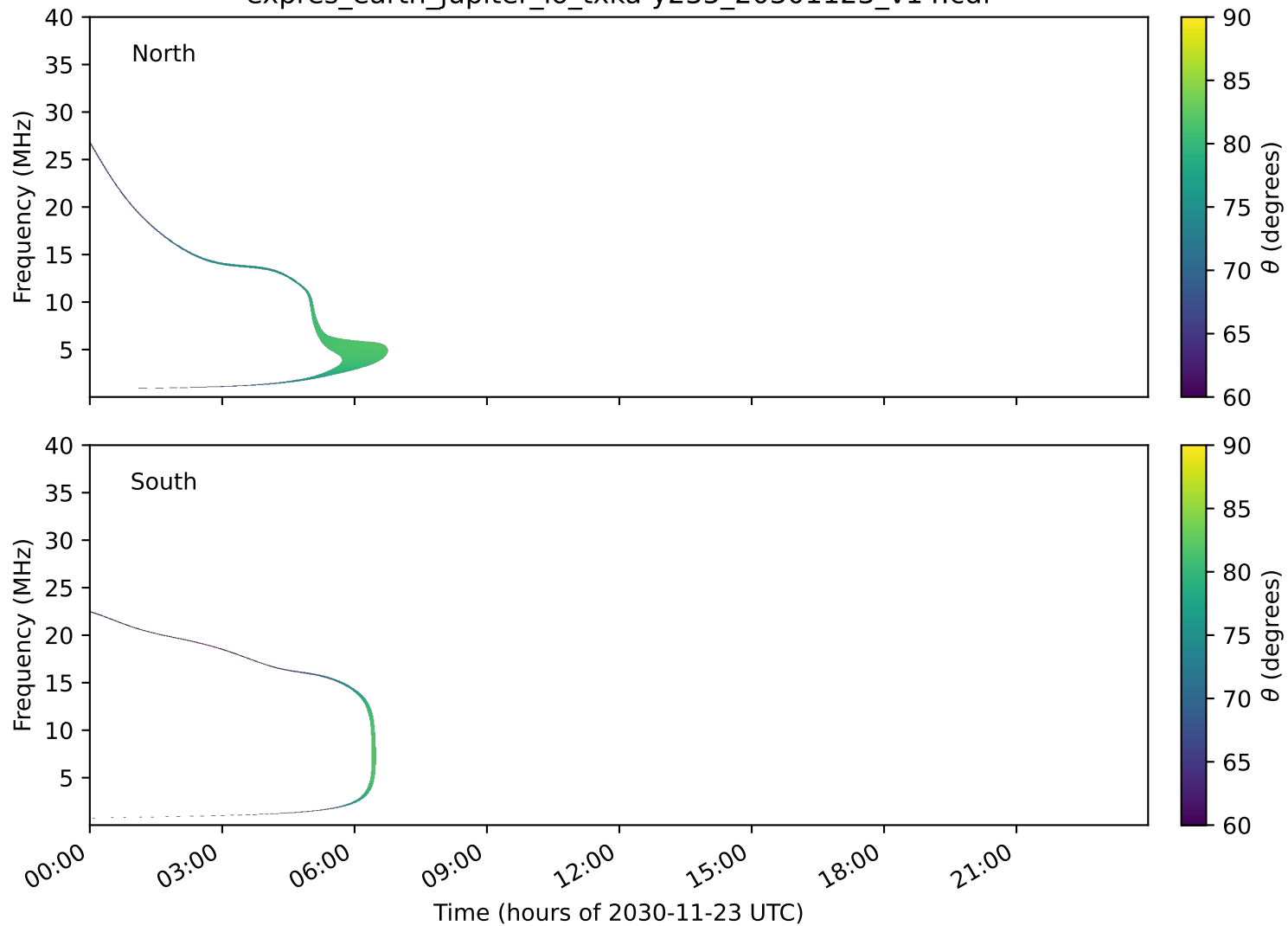
expres_earth_jupiter_io_txka-y235_20301123_v14.cdf
