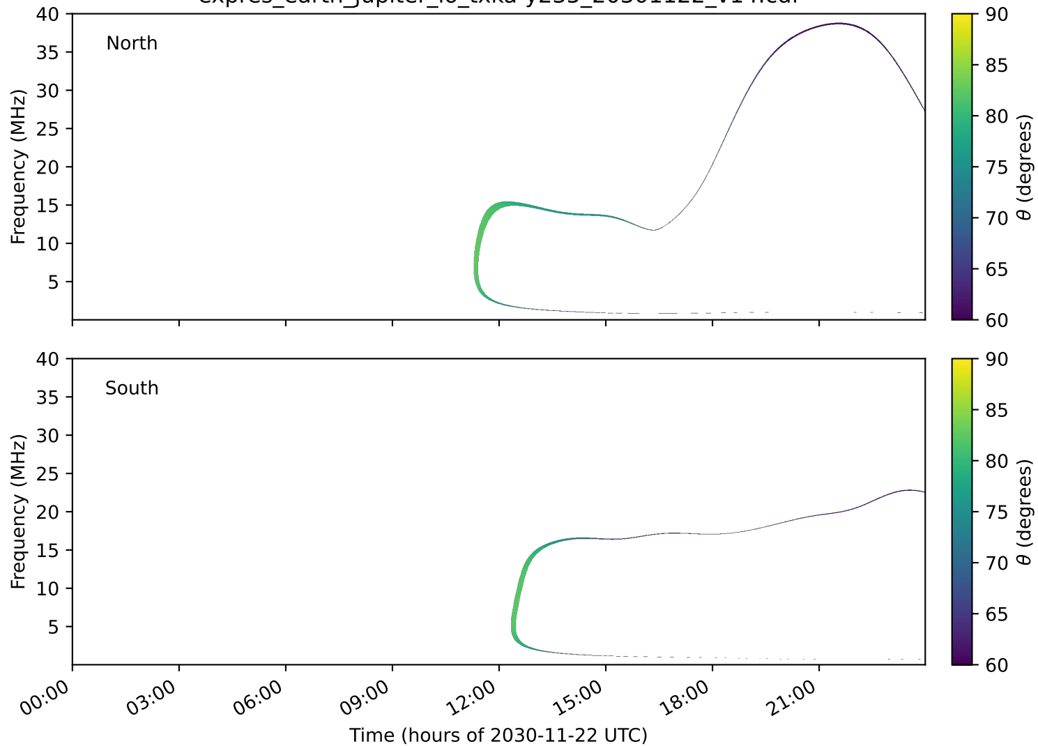
expres_earth_jupiter_io_txka-y235_20301122_v14.cdf
