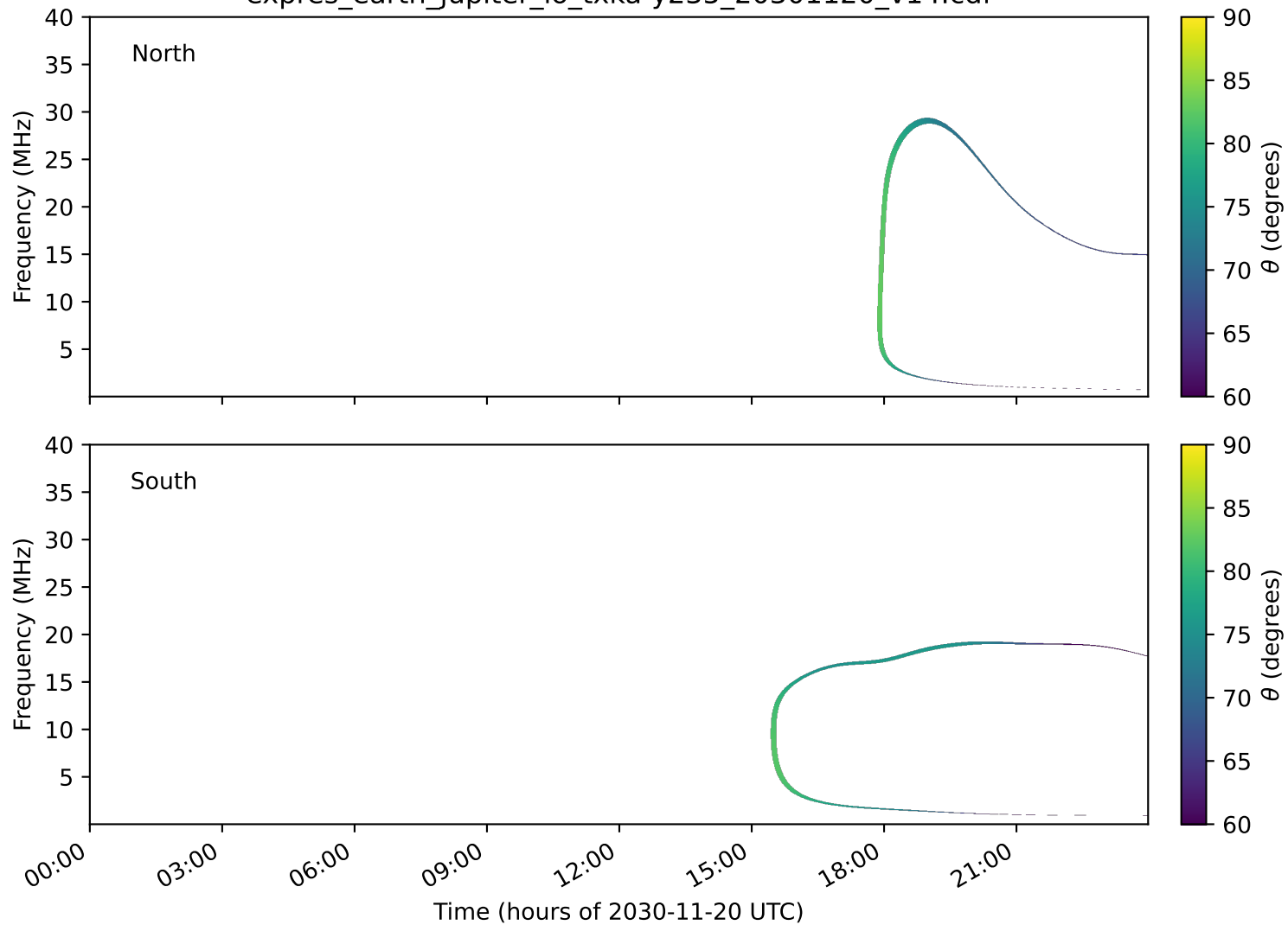
expres_earth_jupiter_io_txka-y235_20301120_v14.cdf
