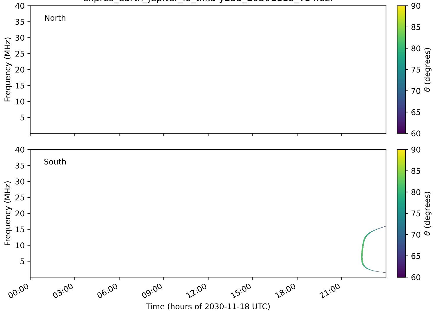
expres_earth_jupiter_io_txka-y235_20301118_v14.cdf
