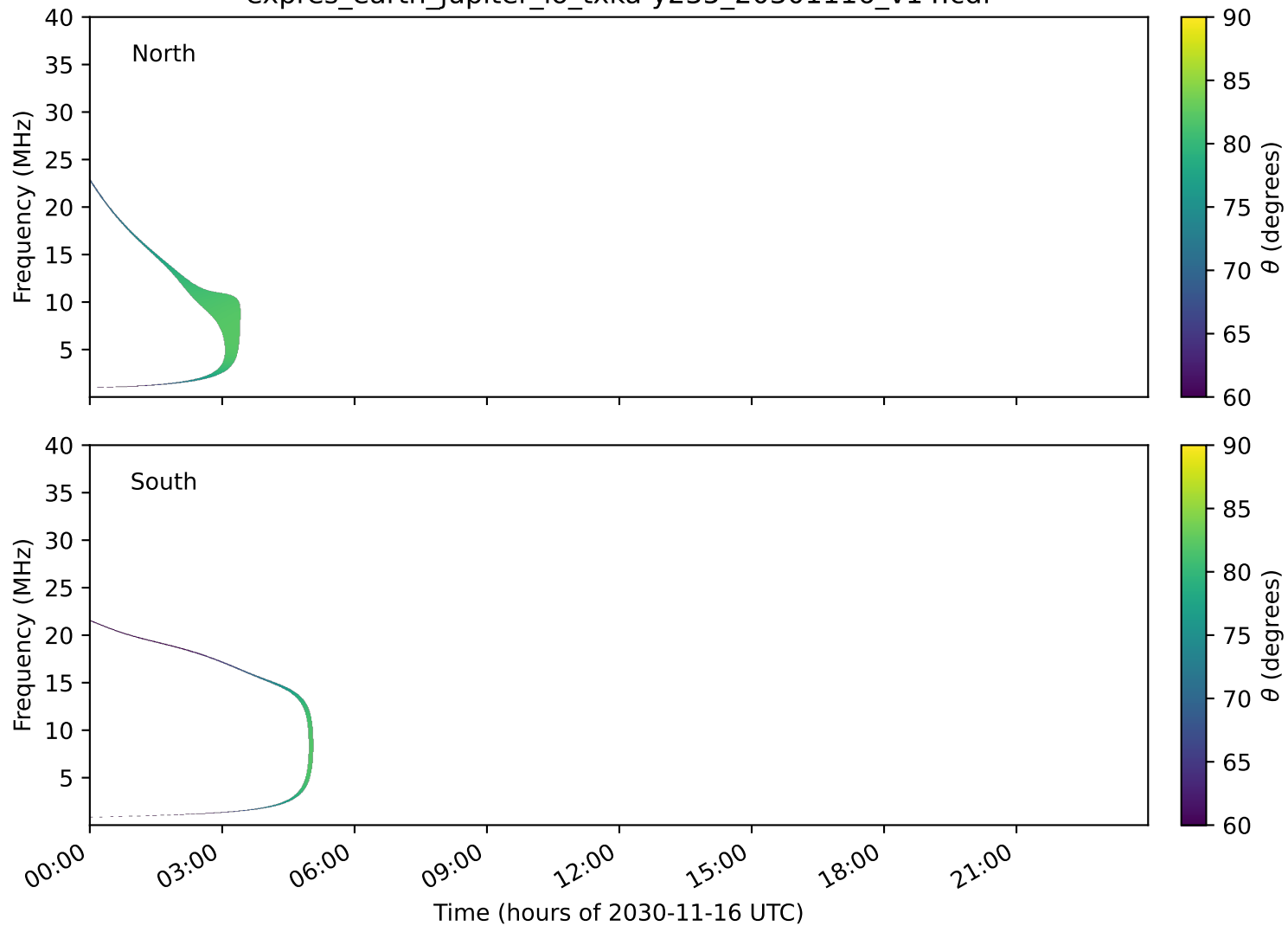
expres_earth_jupiter_io_txka-y235_20301116_v14.cdf
