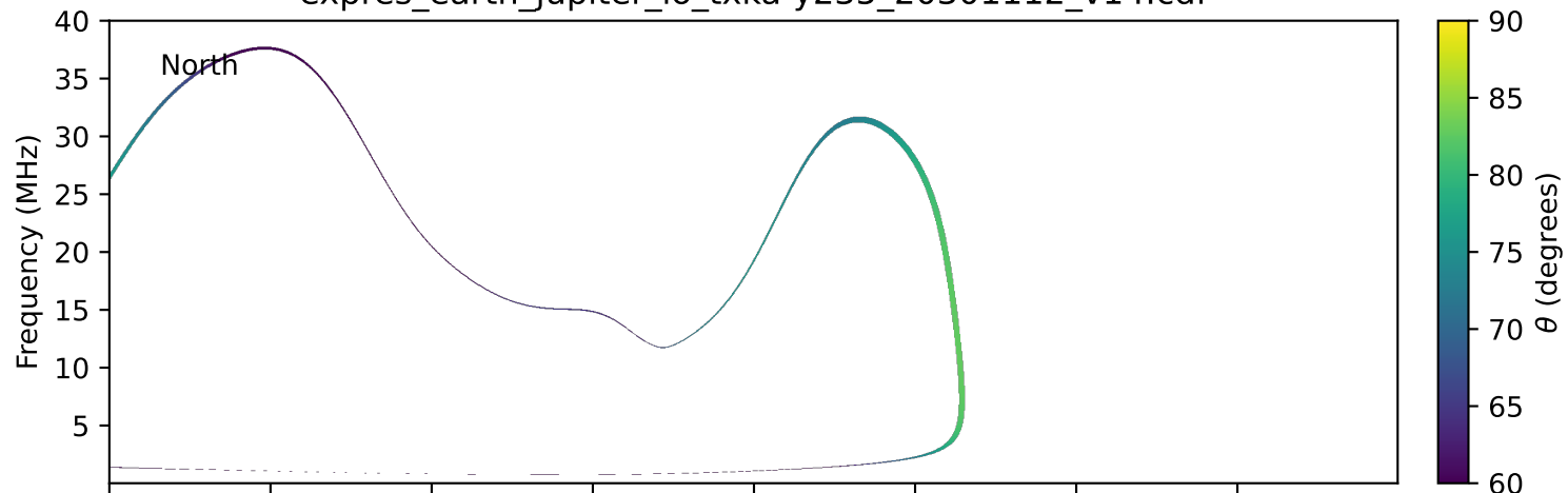
expres_earth_jupiter_io_txka-y235_20301112_v14.cdf
