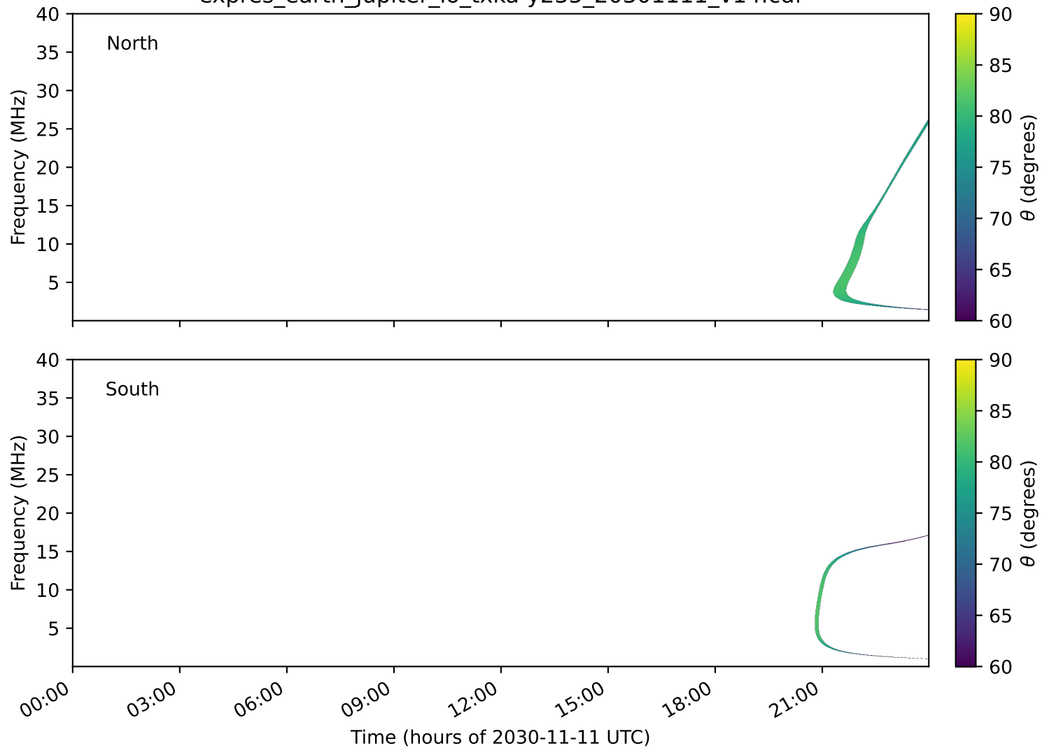
expres_earth_jupiter_io_txka-y235_20301111_v14.cdf
