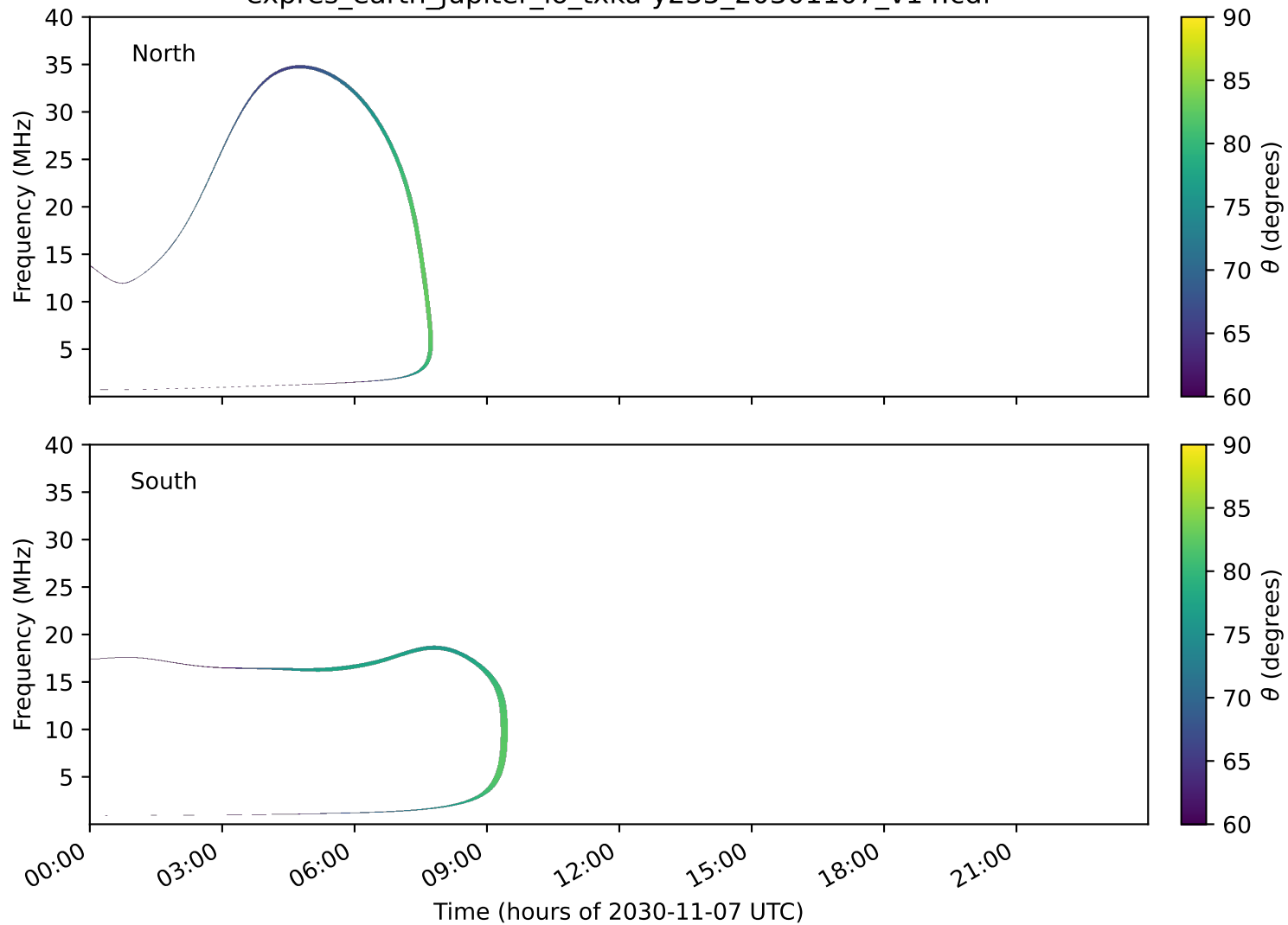
expres_earth_jupiter_io_txka-y235_20301107_v14.cdf
