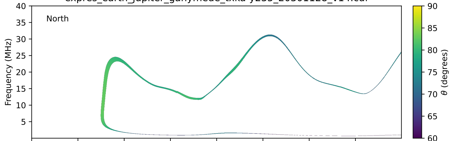
expres_earth_jupiter_ganymede_txka-y235_20301128_v14.cdf
