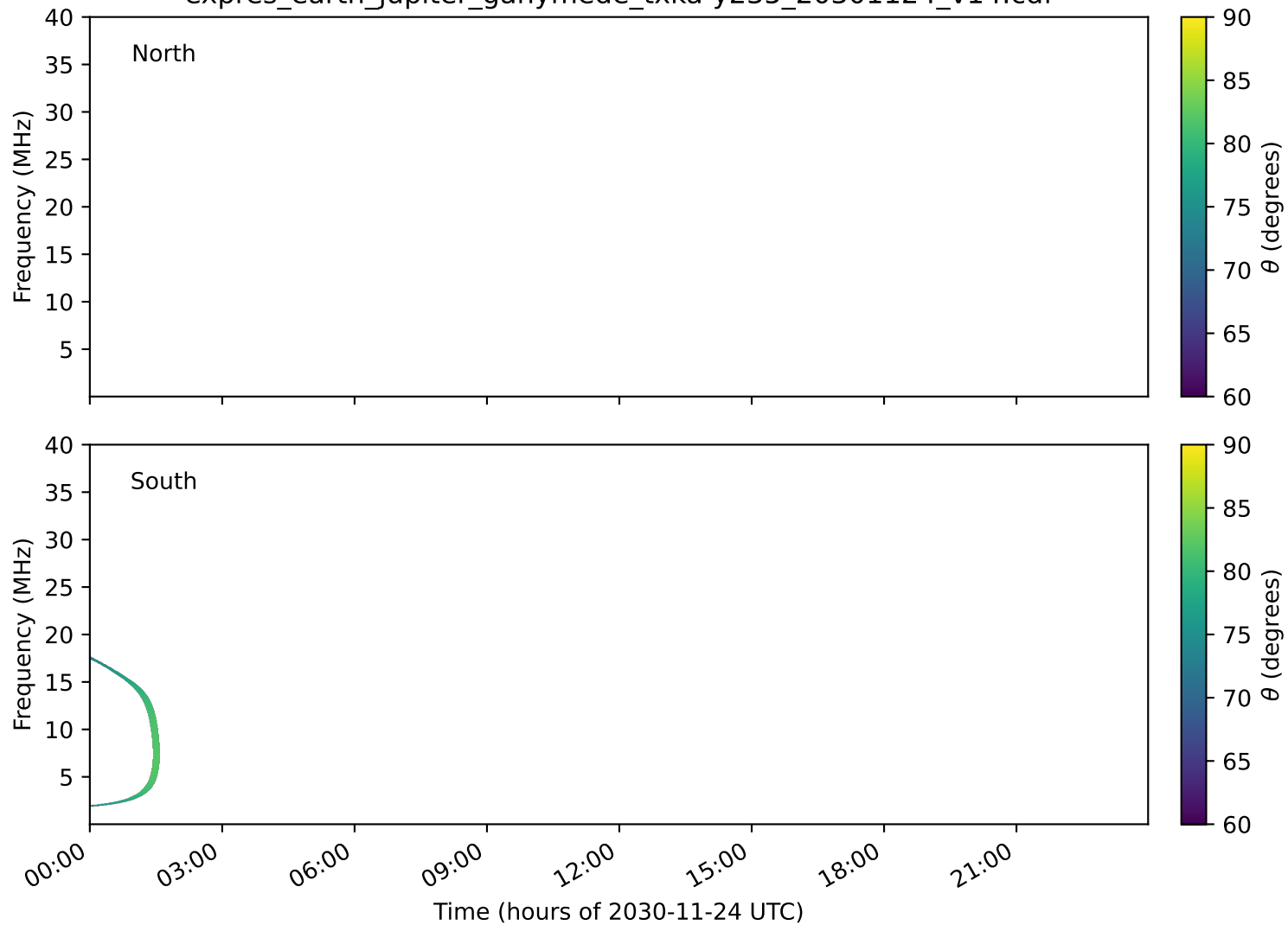
expres_earth_jupiter_ganymede_txka-y235_20301124_v14.cdf
