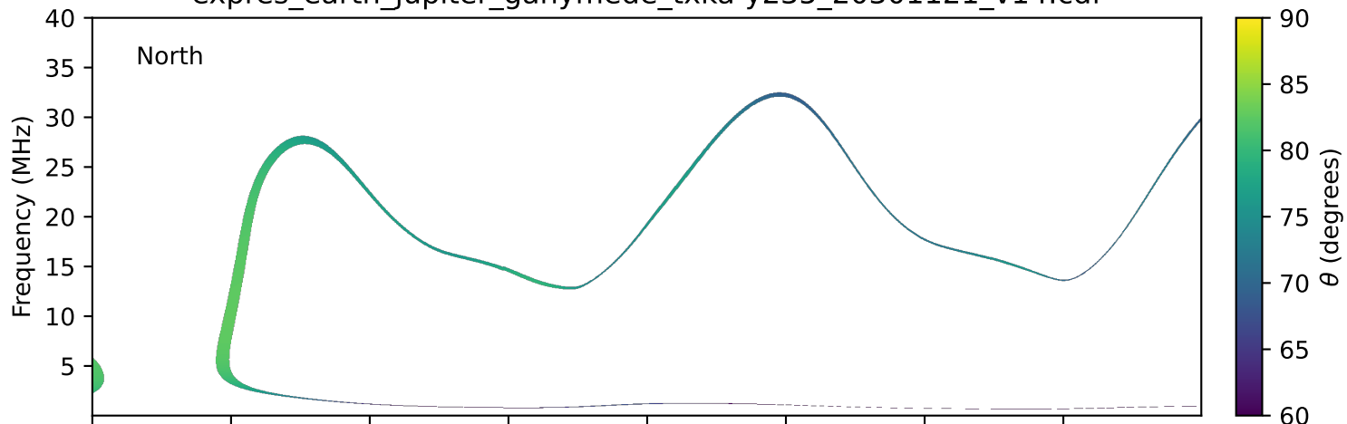
expres_earth_jupiter_ganymede_txka-y235_20301121_v14.cdf
