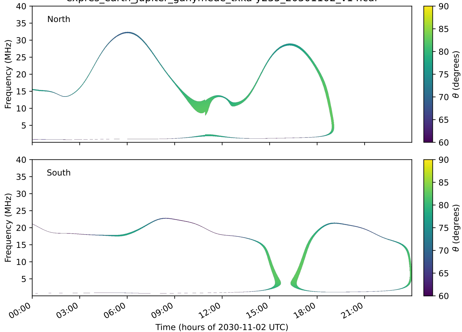
expres_earth_jupiter_ganymede_txka-y235_20301102_v14.cdf
