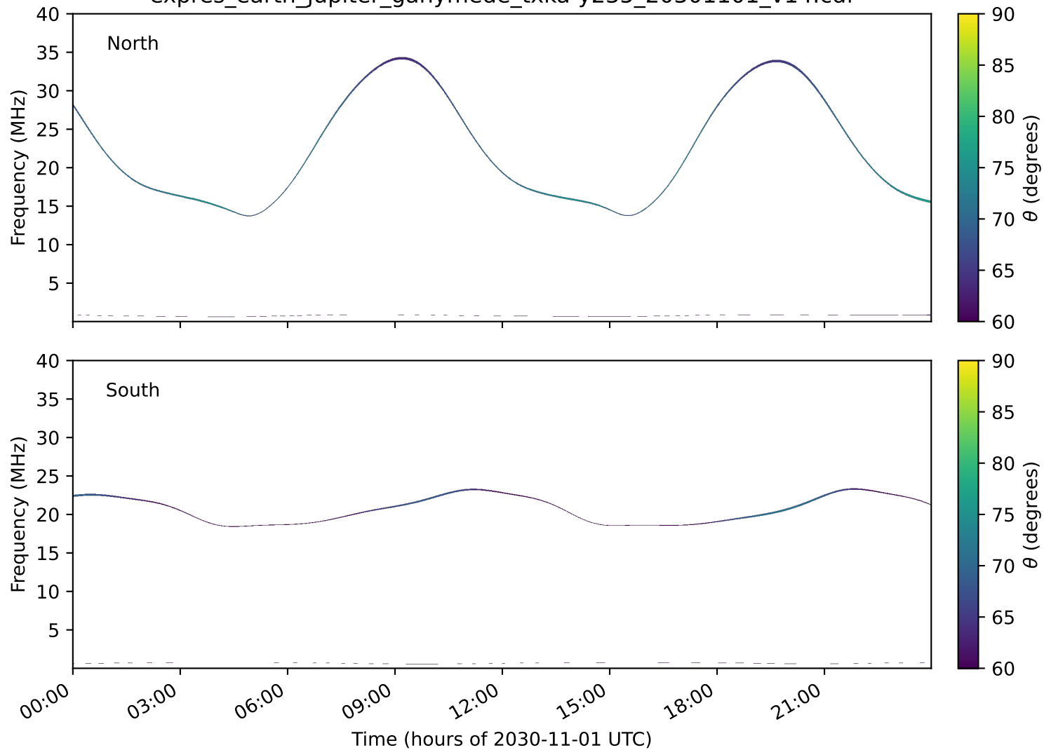
expres_earth_jupiter_ganymede_txka-y235_20301101_v14.cdf
