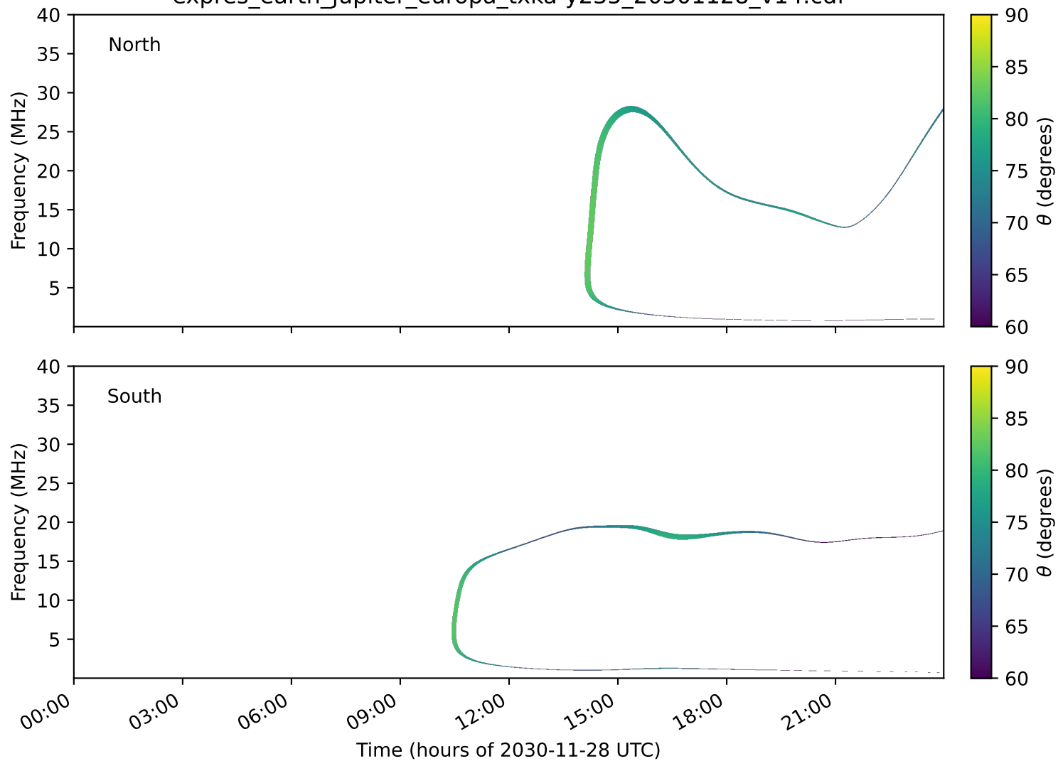
expres_earth_jupiter_europa_txka-y235_20301128_v14.cdf
