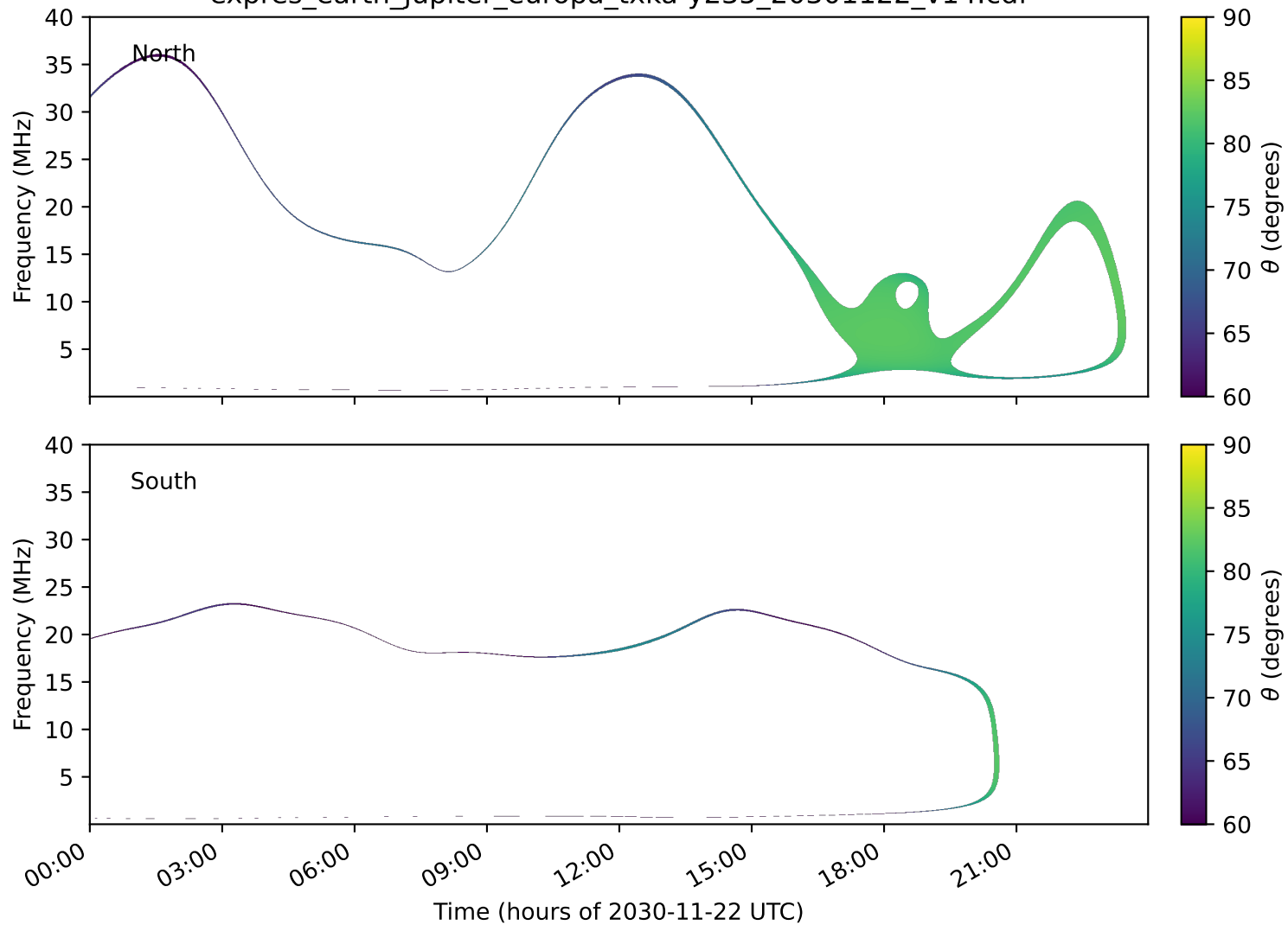
expres_earth_jupiter_europa_txka-y235_20301122_v14.cdf
