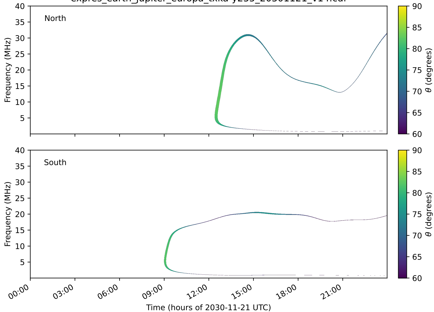
expres_earth_jupiter_europa_txka-y235_20301121_v14.cdf
