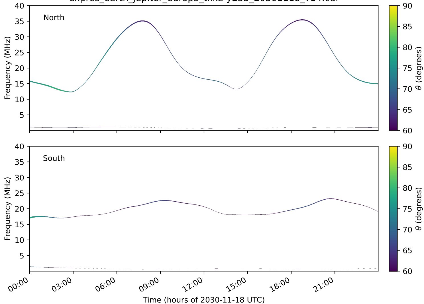
expres_earth_jupiter_europa_txka-y235_20301118_v14.cdf
