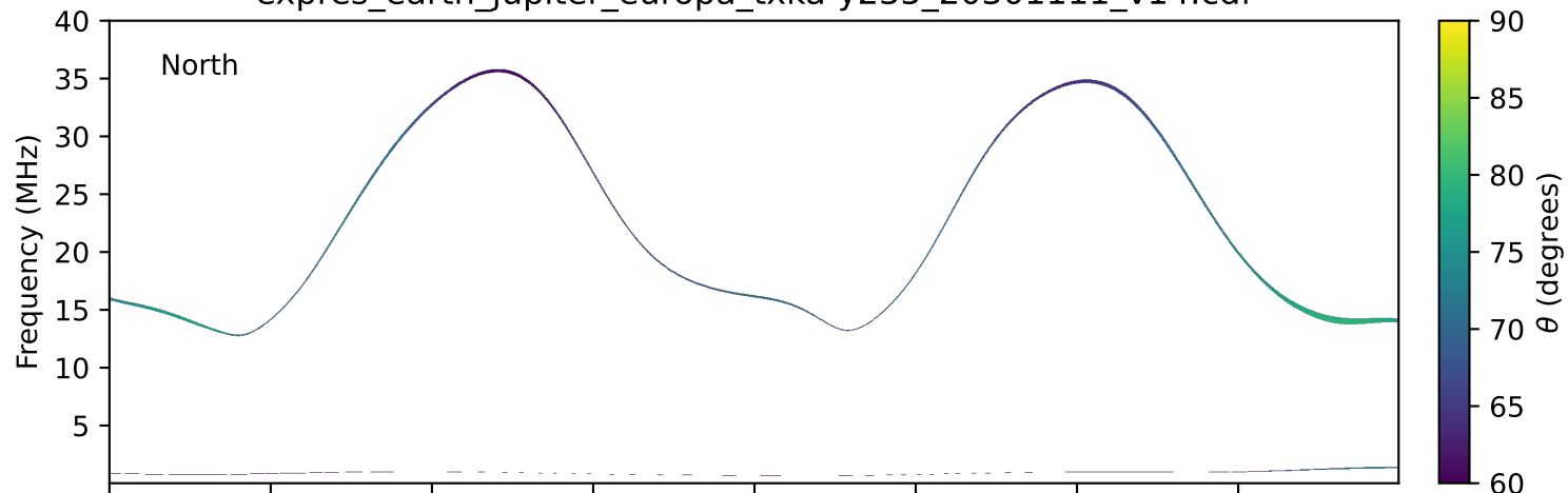
expres_earth_jupiter_europa_txka-y235_20301111_v14.cdf
