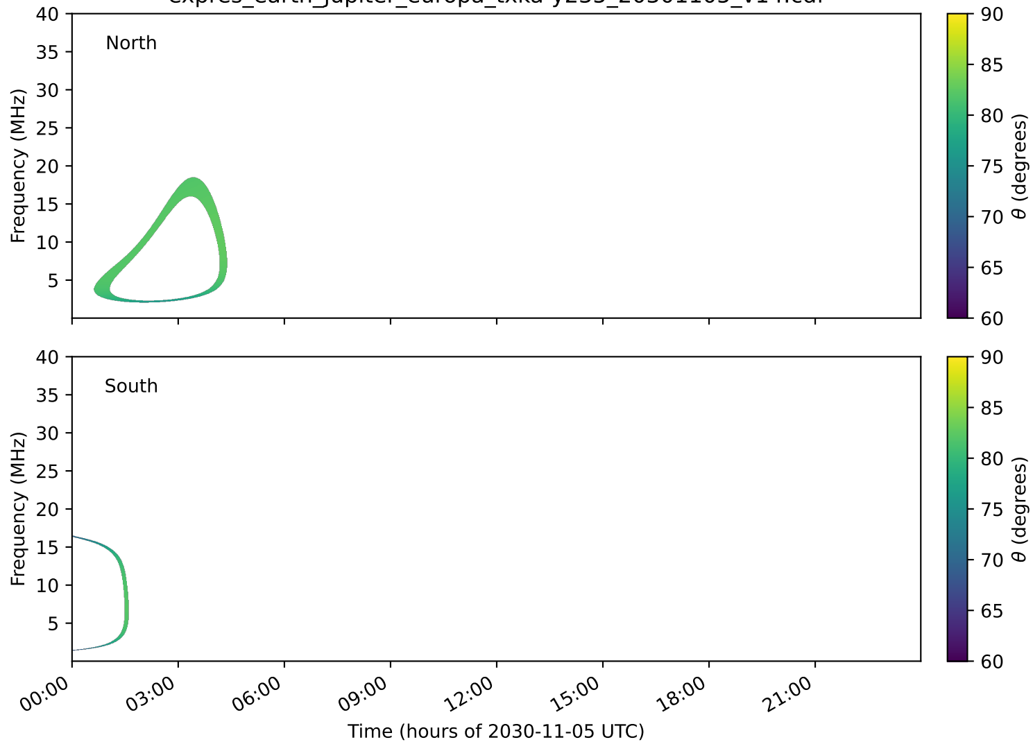
expres_earth_jupiter_europa_txka-y235_20301105_v14.cdf
