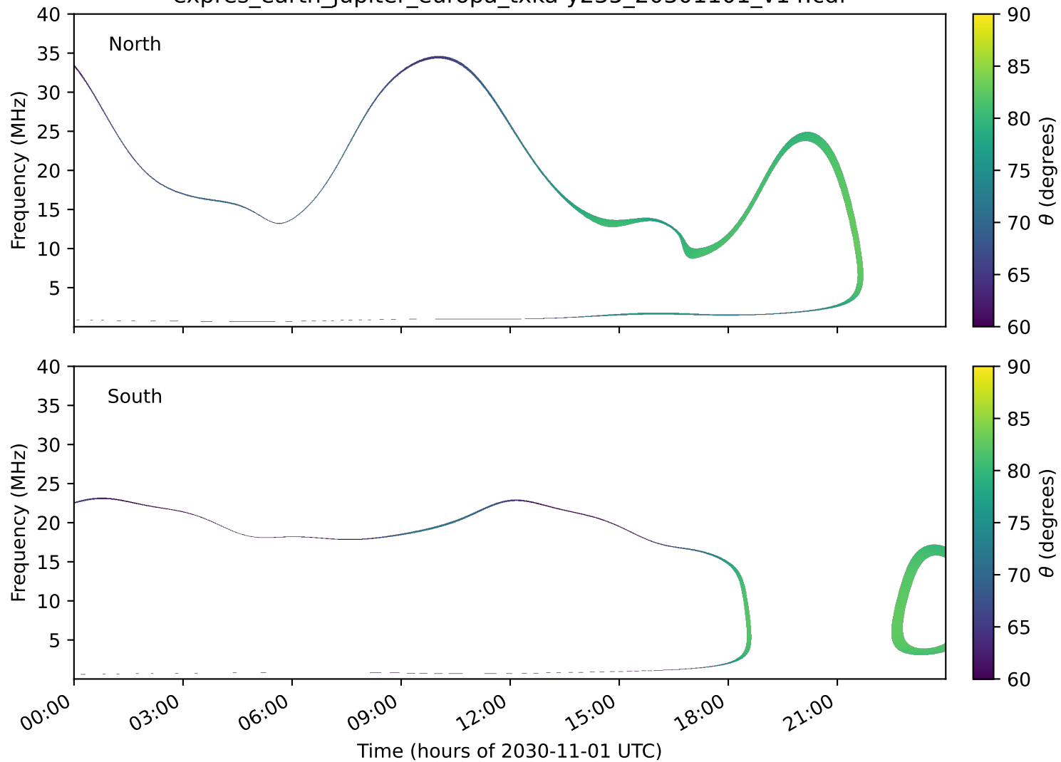
expres_earth_jupiter_europa_txka-y235_20301101_v14.cdf
