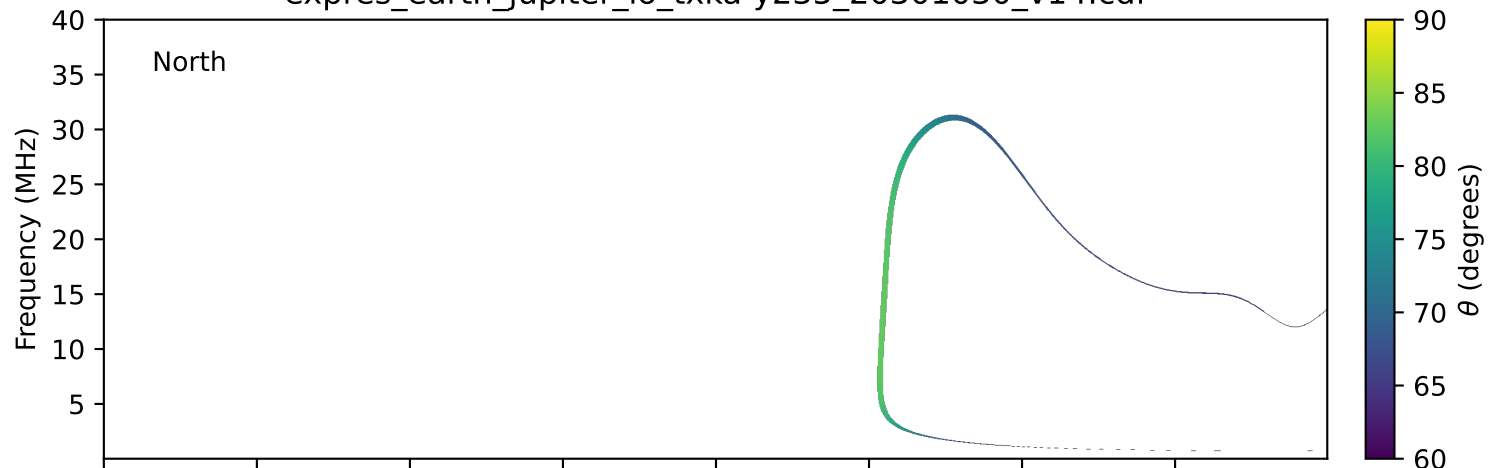
expres_earth_jupiter_io_txka-y235_20301030_v14.cdf
