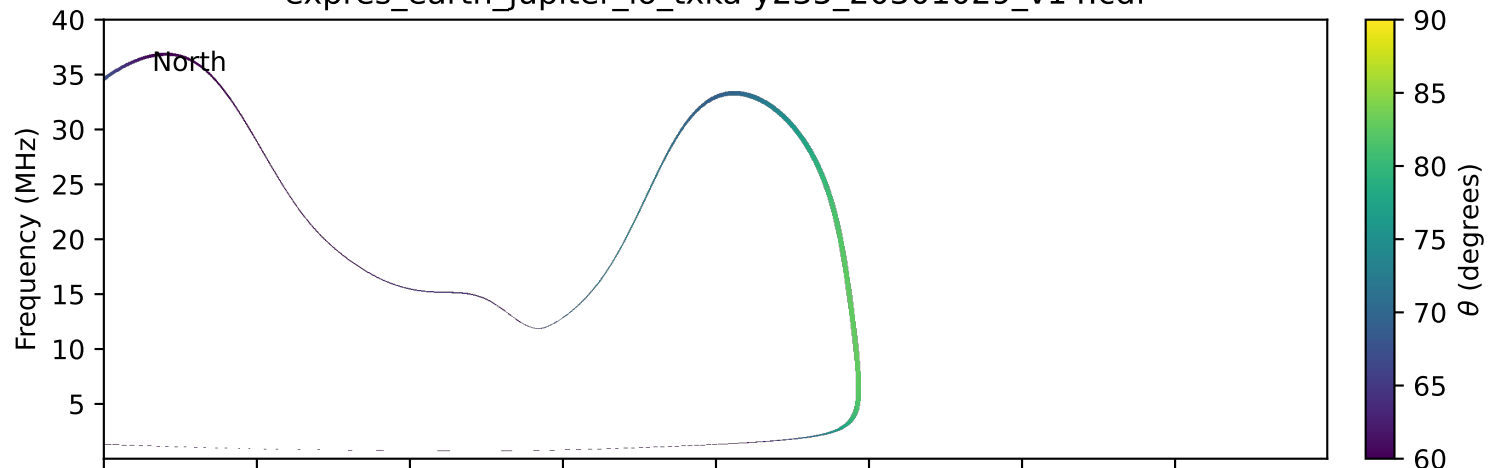
expres_earth_jupiter_io_txka-y235_20301029_v14.cdf
