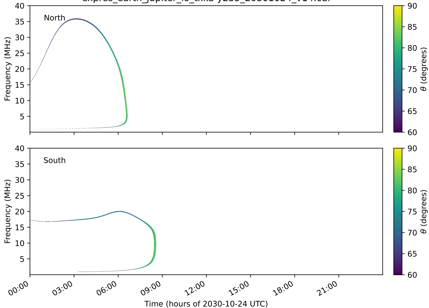
expres_earth_jupiter_io_txka-y235_20301024_v14.cdf
