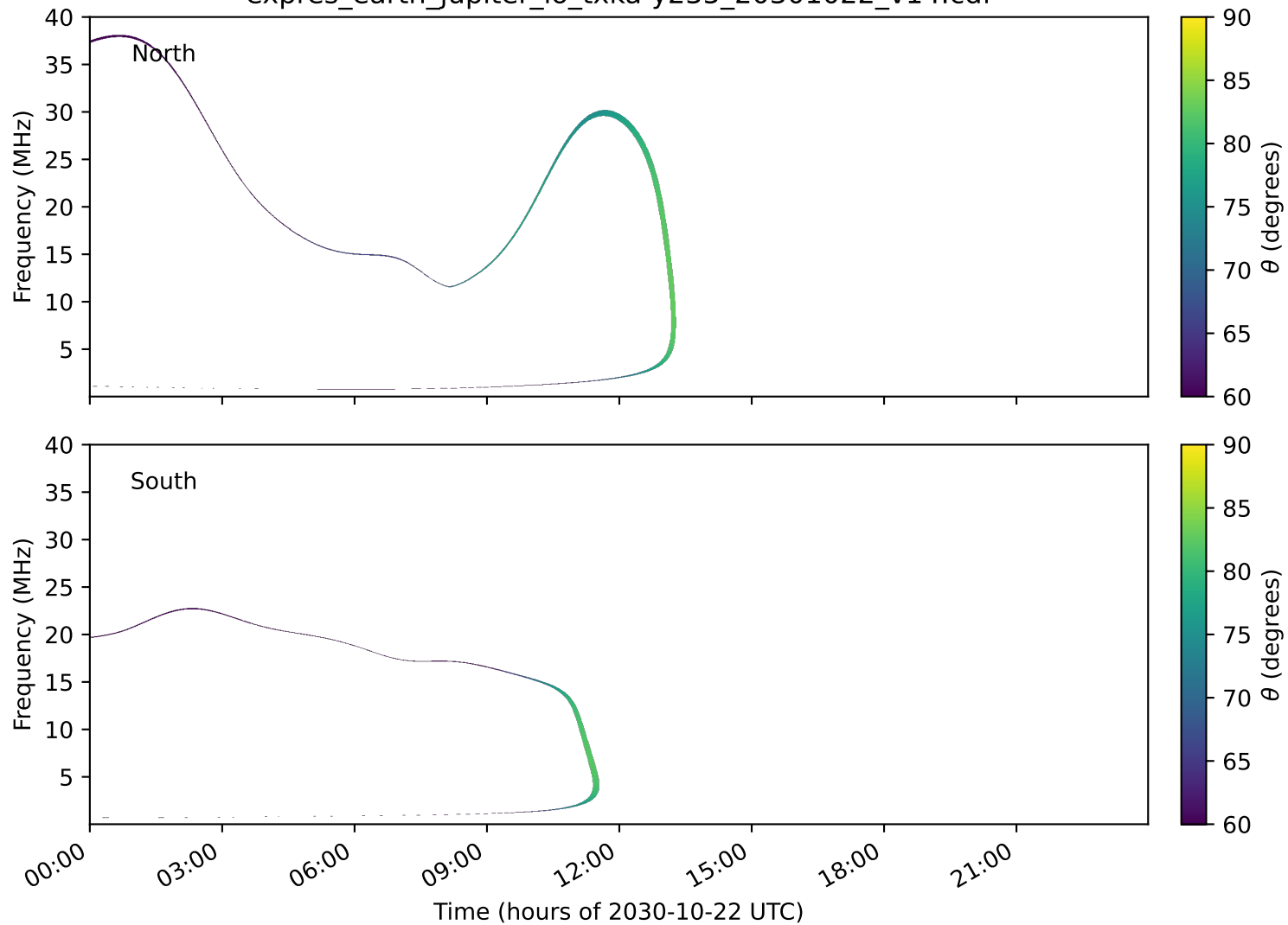
expres_earth_jupiter_io_txka-y235_20301022_v14.cdf
