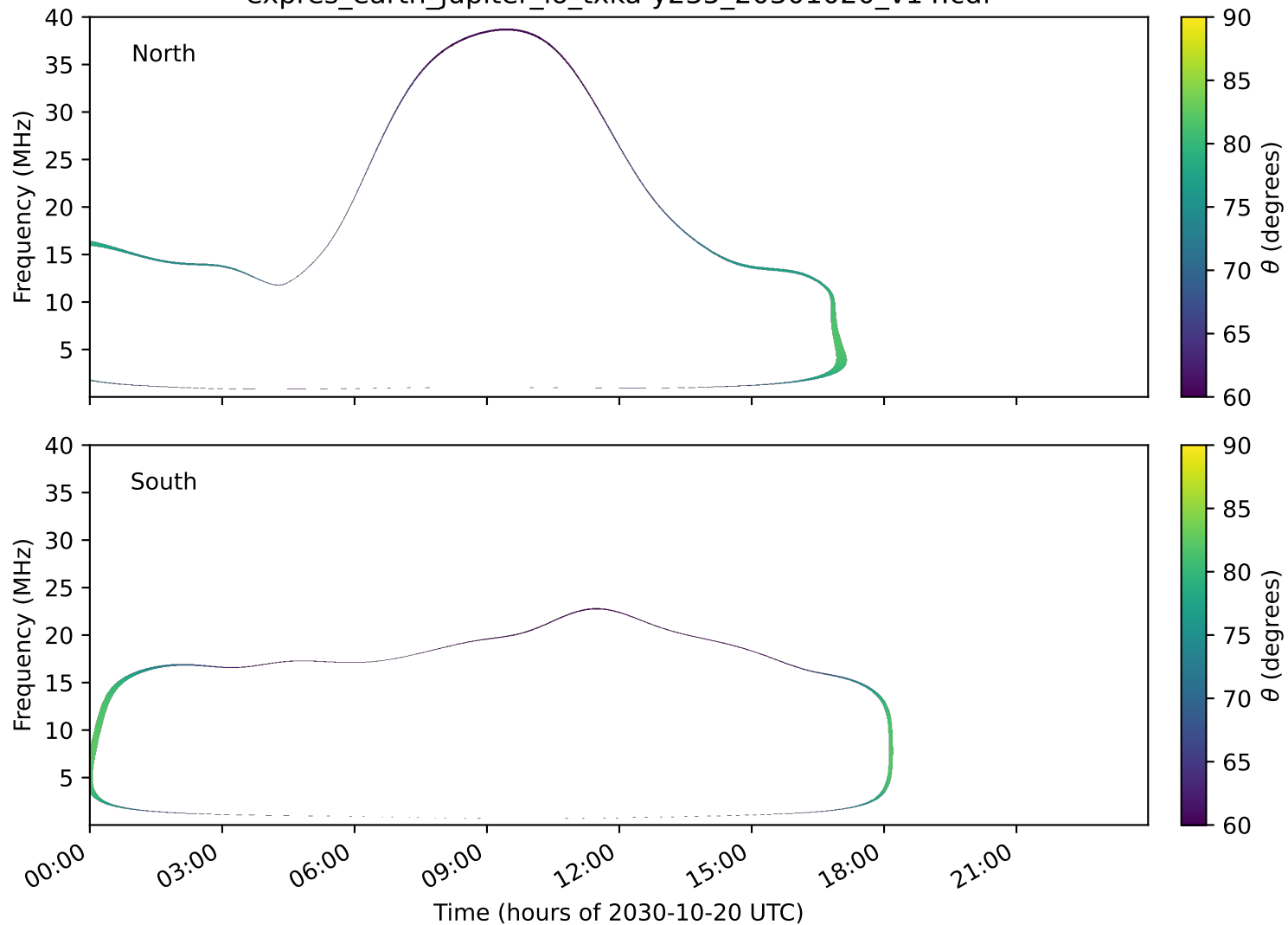
expres_earth_jupiter_io_txka-y235_20301020_v14.cdf
