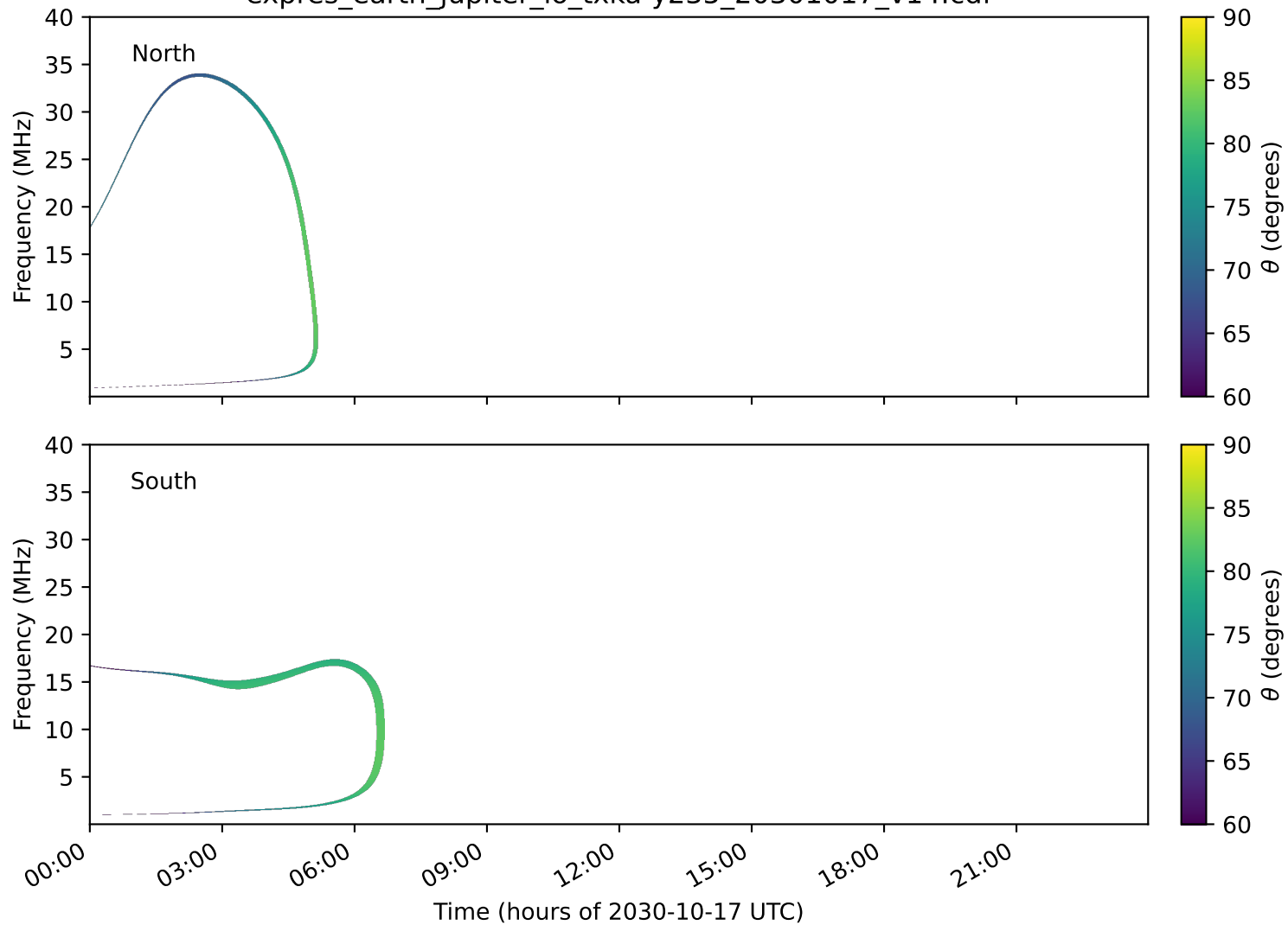
expres_earth_jupiter_io_txka-y235_20301017_v14.cdf
