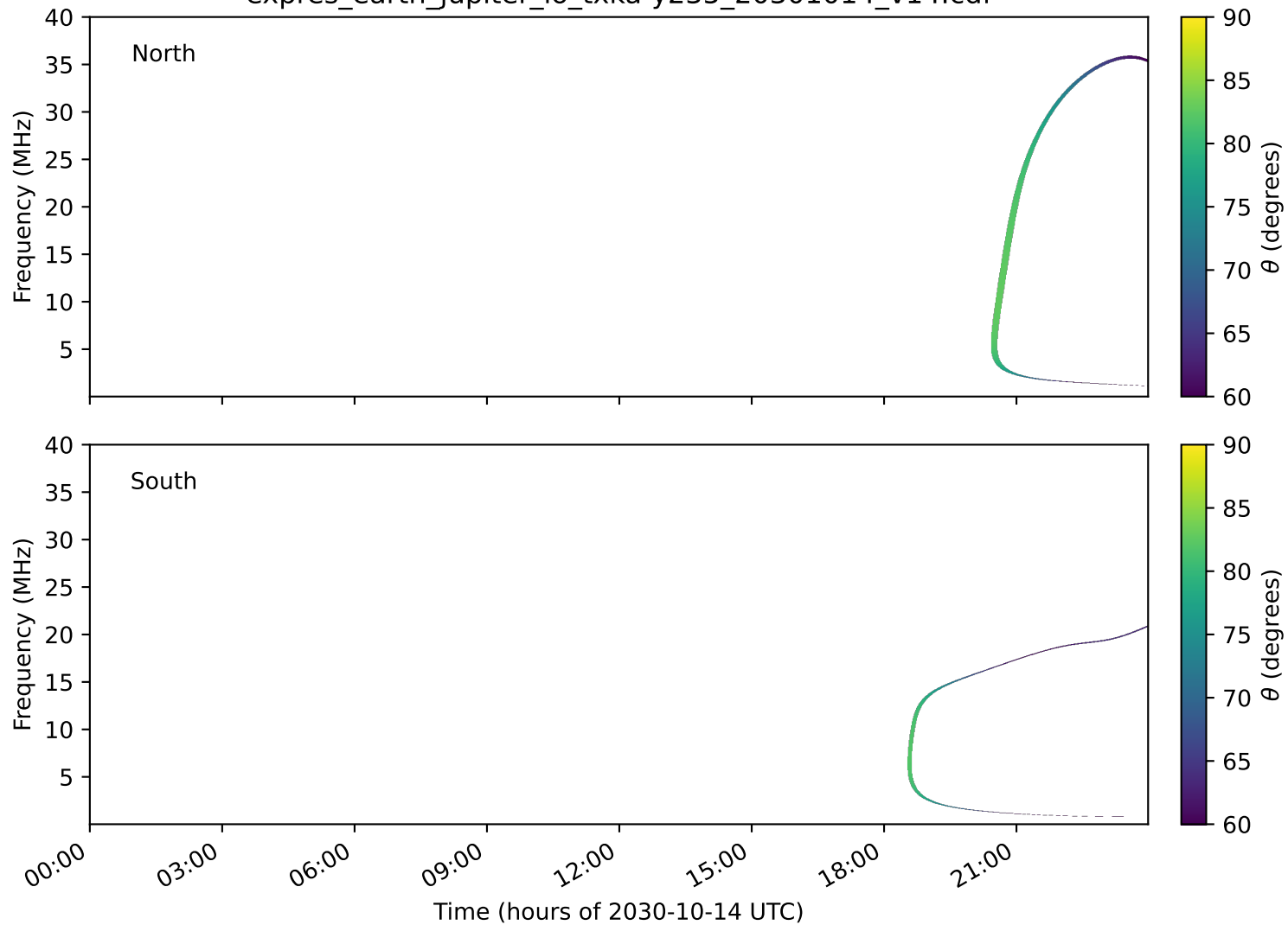
expres_earth_jupiter_io_txka-y235_20301014_v14.cdf
