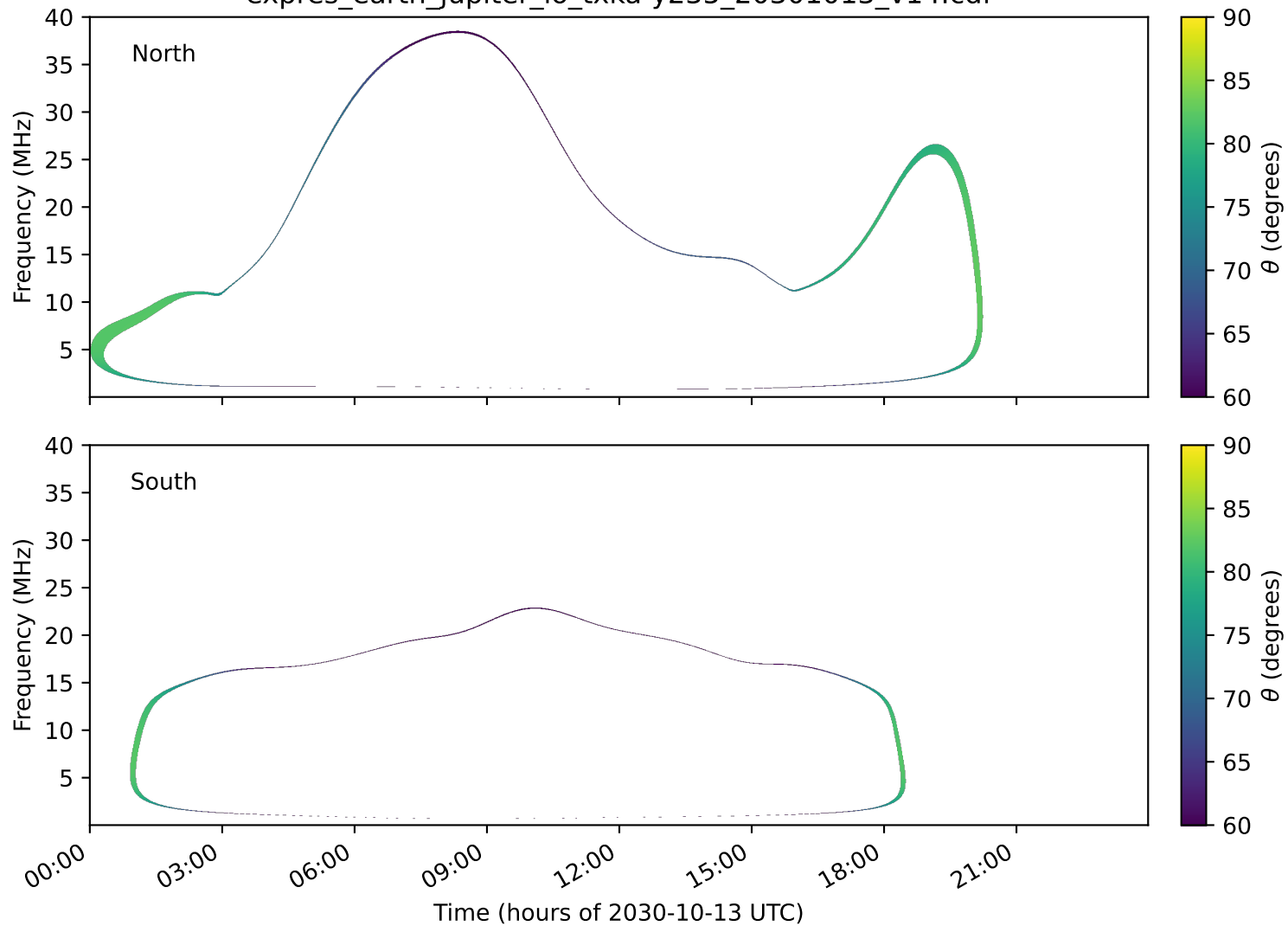
expres_earth_jupiter_io_txka-y235_20301013_v14.cdf
