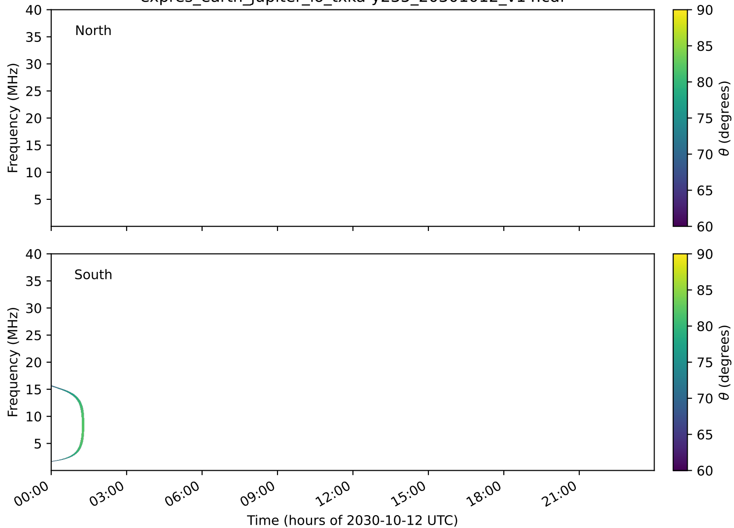
expres_earth_jupiter_io_txka-y235_20301012_v14.cdf
