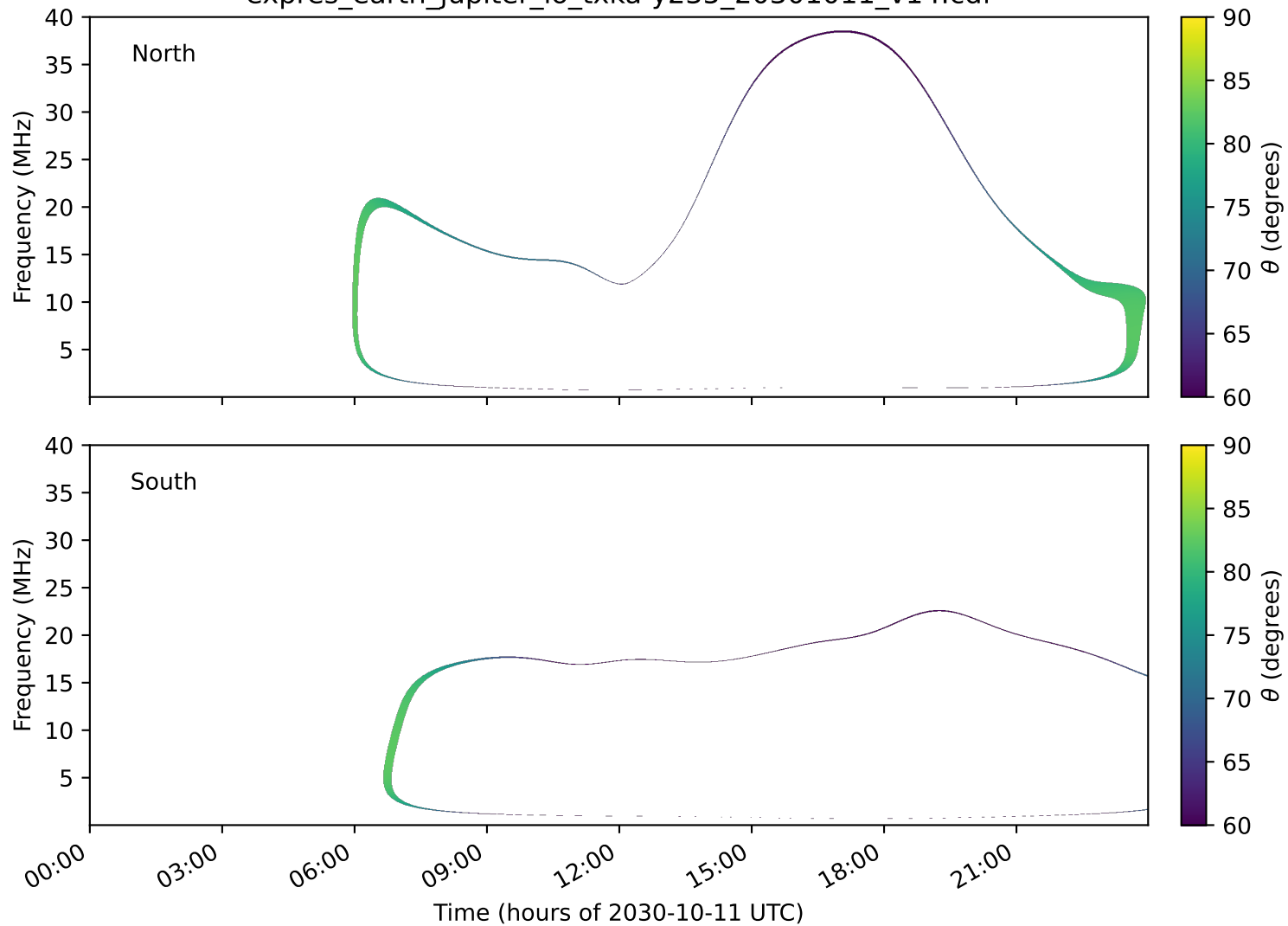
expres_earth_jupiter_io_txka-y235_20301011_v14.cdf
