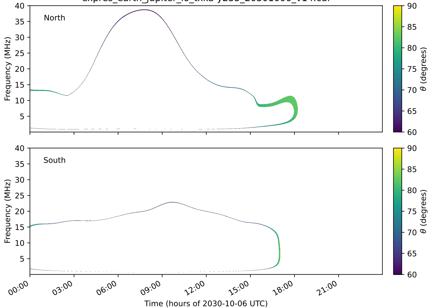
expres_earth_jupiter_io_txka-y235_20301006_v14.cdf
