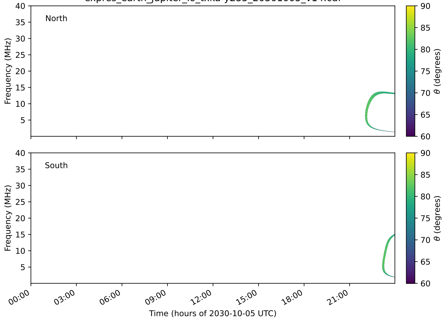
expres_earth_jupiter_io_txka-y235_20301005_v14.cdf
