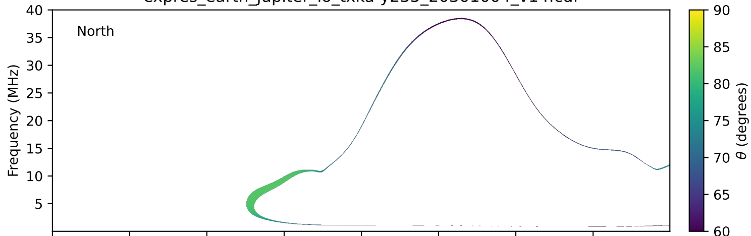
expres_earth_jupiter_io_txka-y235_20301004_v14.cdf
