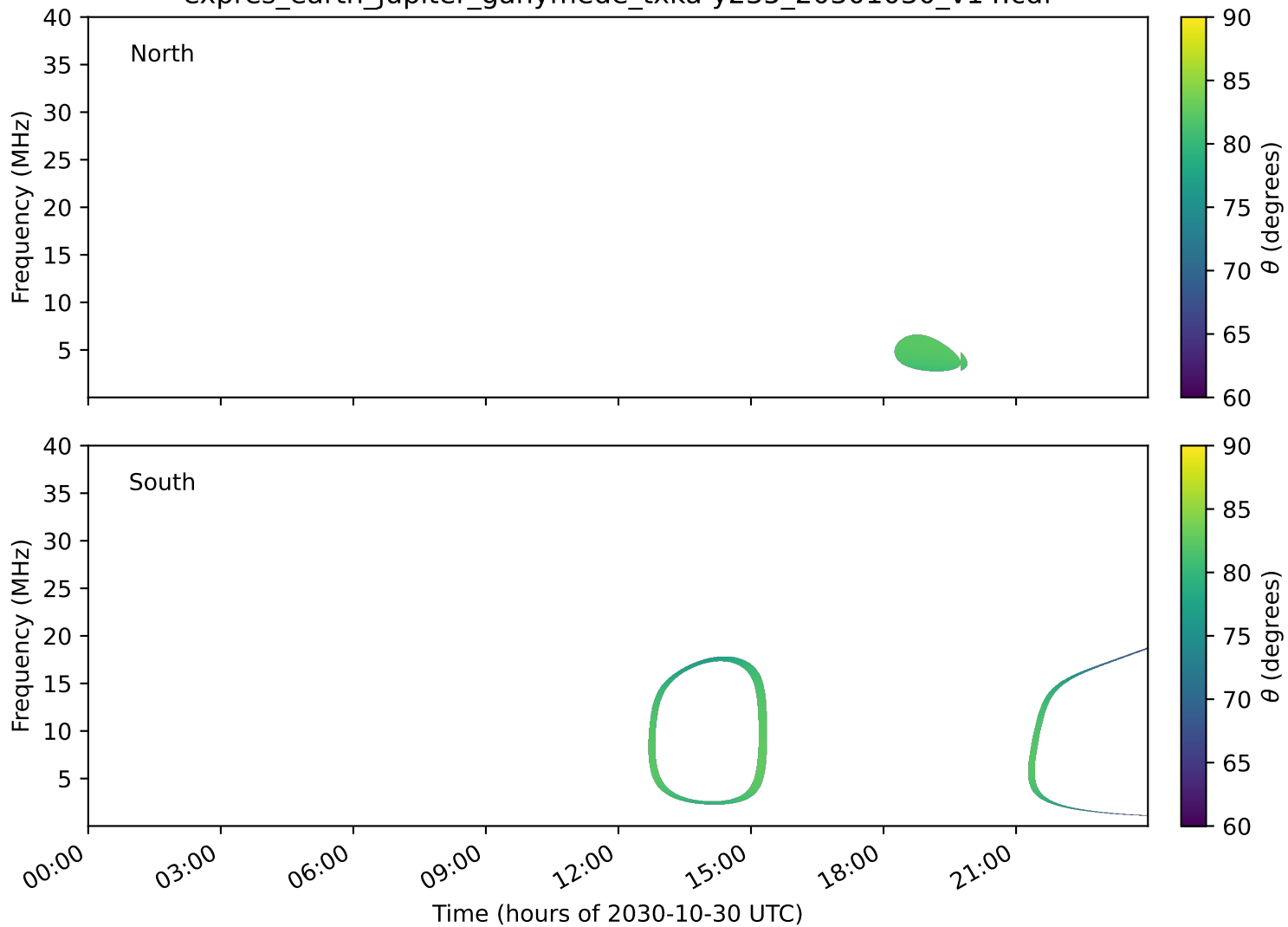
expres_earth_jupiter_ganymede_txka-y235_20301030_v14.cdf
