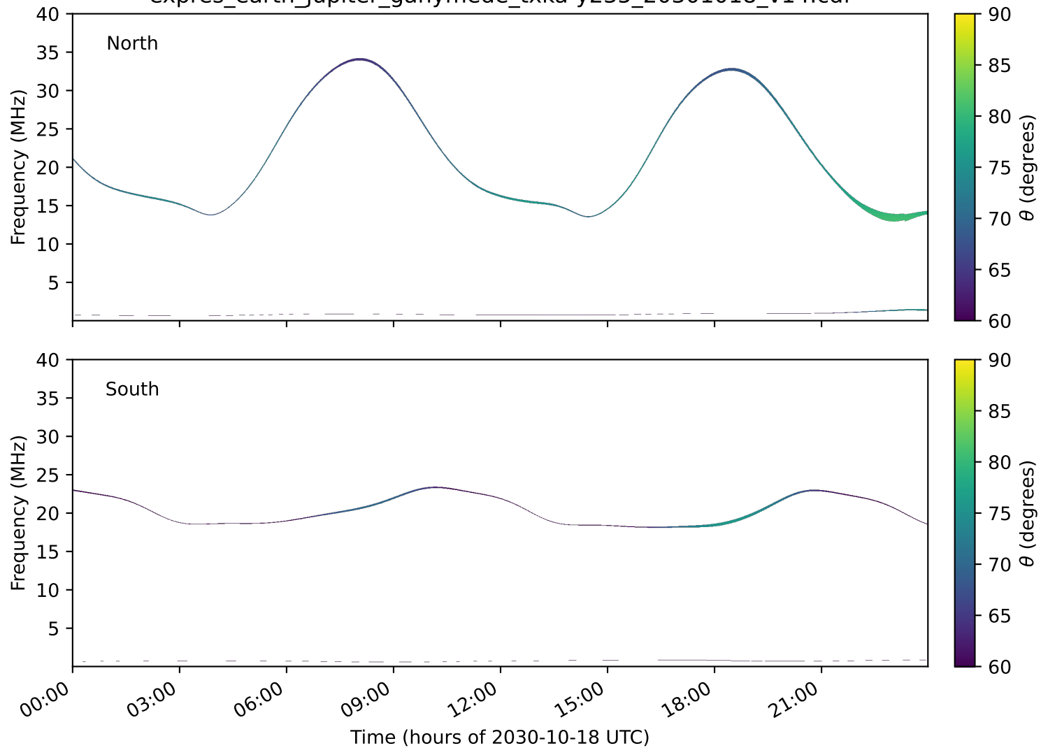
expres_earth_jupiter_ganymede_txka-y235_20301018_v14.cdf
