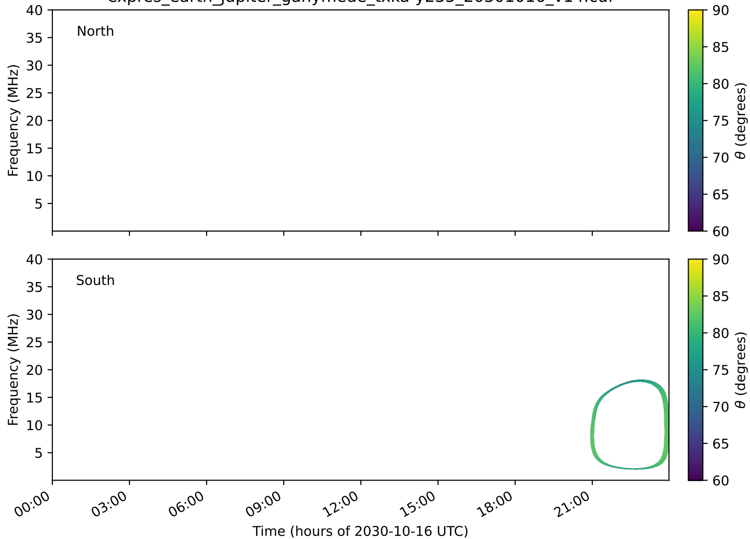
expres_earth_jupiter_ganymede_txka-y235_20301016_v14.cdf
