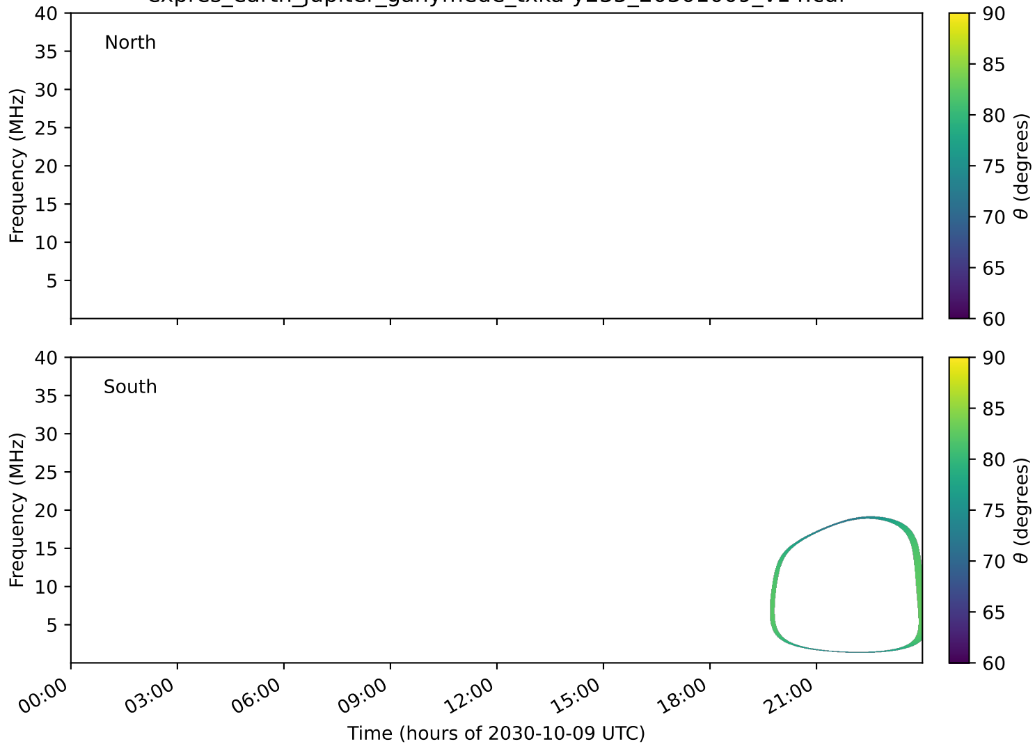
expres_earth_jupiter_ganymede_txka-y235_20301009_v14.cdf
