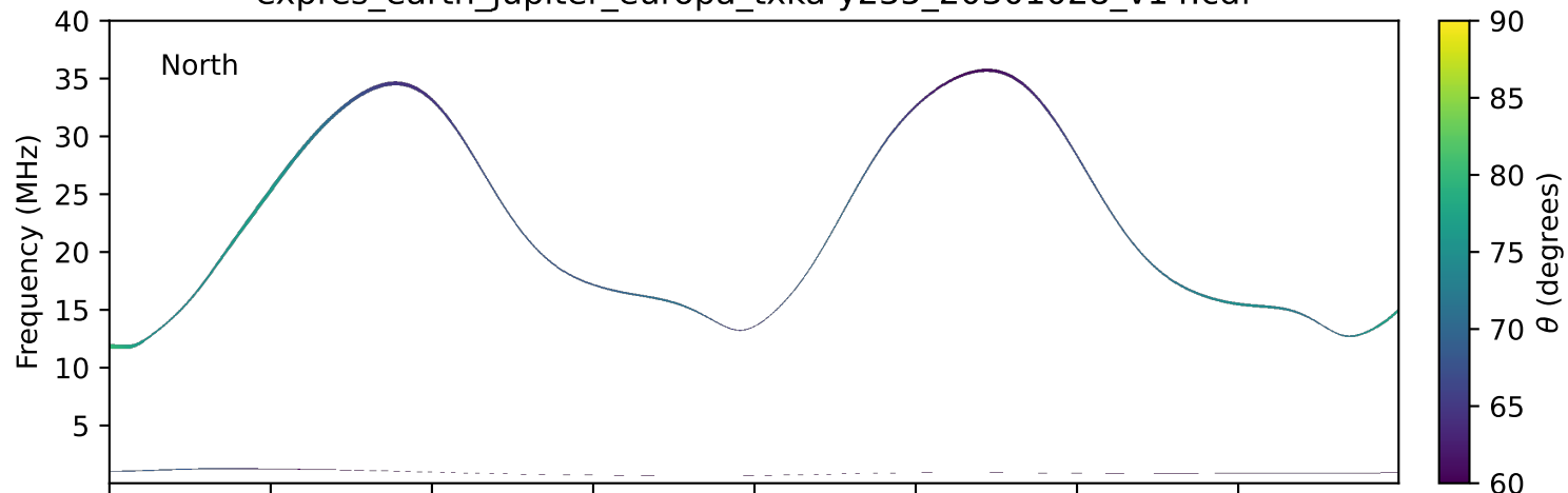
expres_earth_jupiter_europa_txka-y235_20301028_v14.cdf
