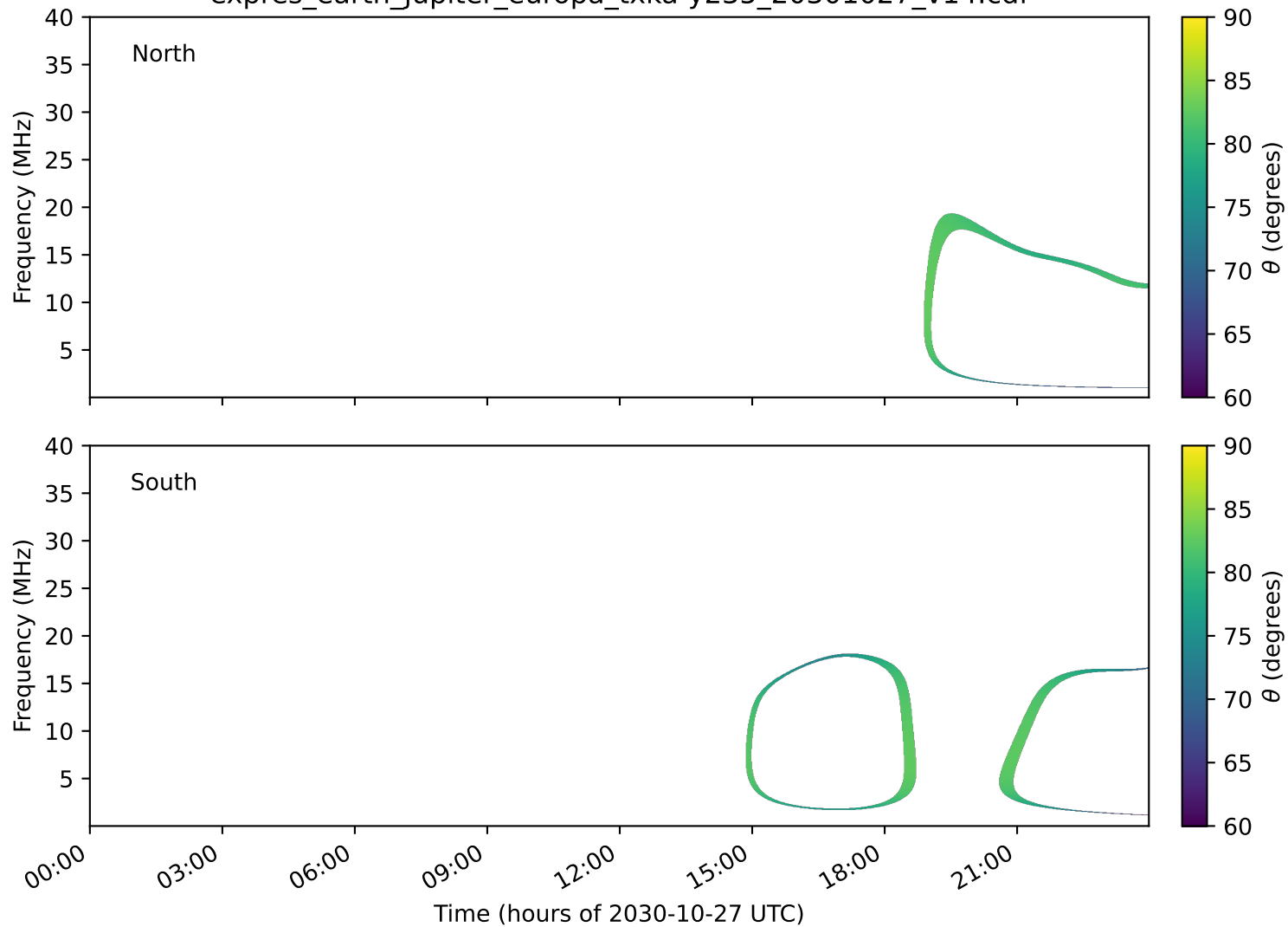
expres_earth_jupiter_europa_txka-y235_20301027_v14.cdf
