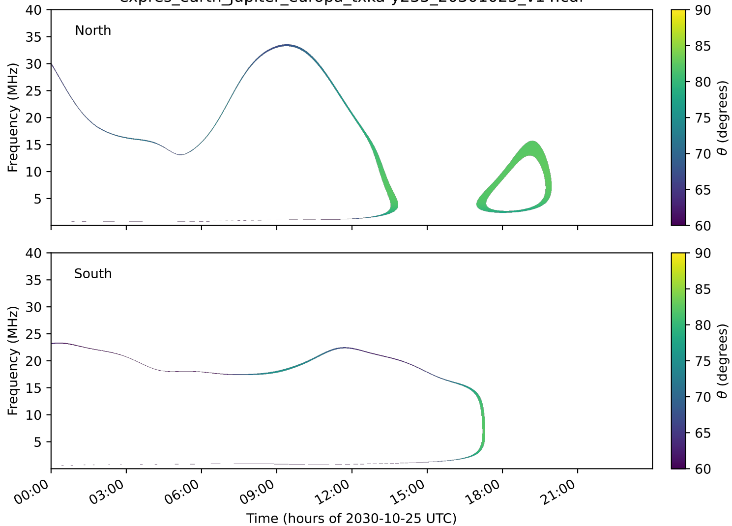
expres_earth_jupiter_europa_txka-y235_20301025_v14.cdf
