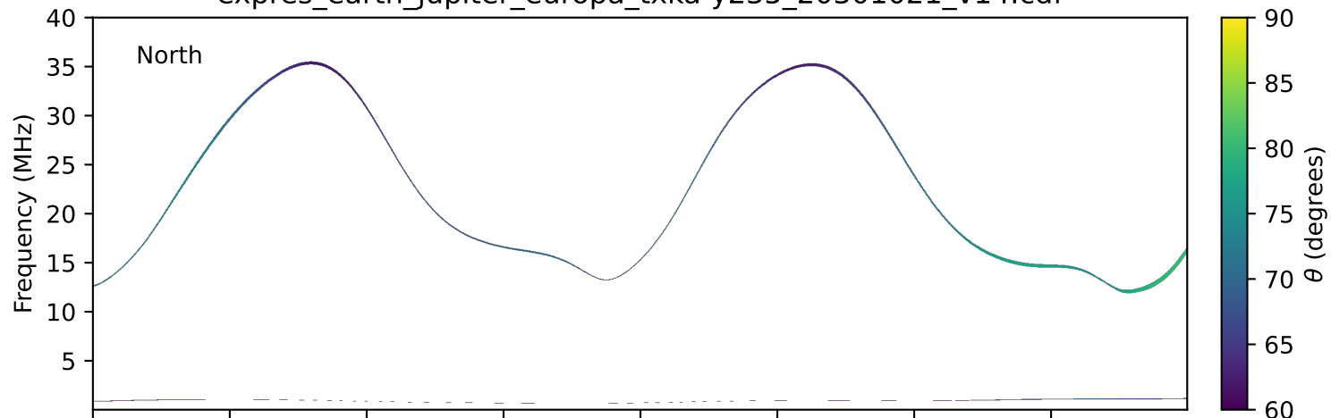
expres_earth_jupiter_europa_txka-y235_20301021_v14.cdf
