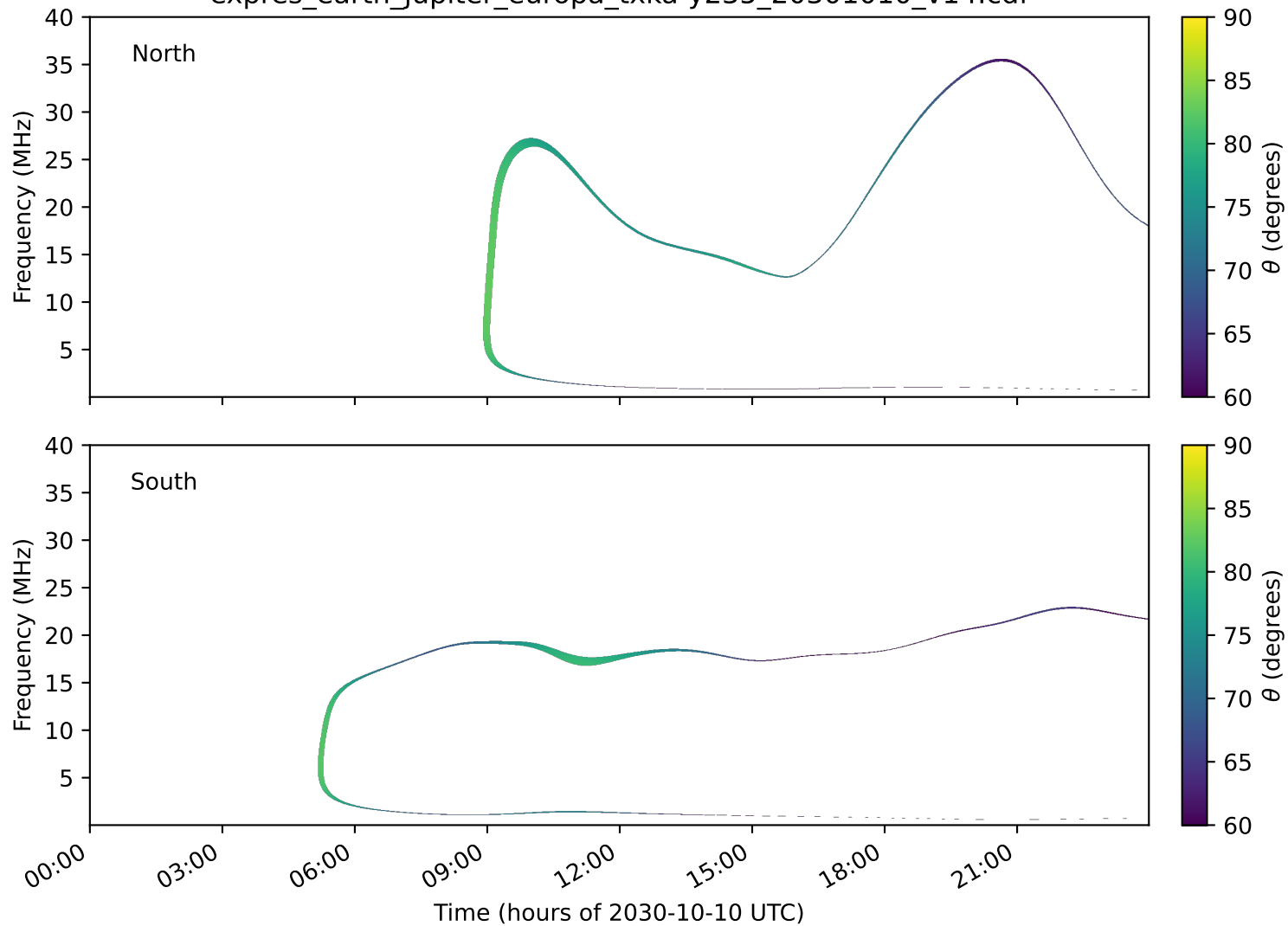
expres_earth_jupiter_europa_txka-y235_20301010_v14.cdf
