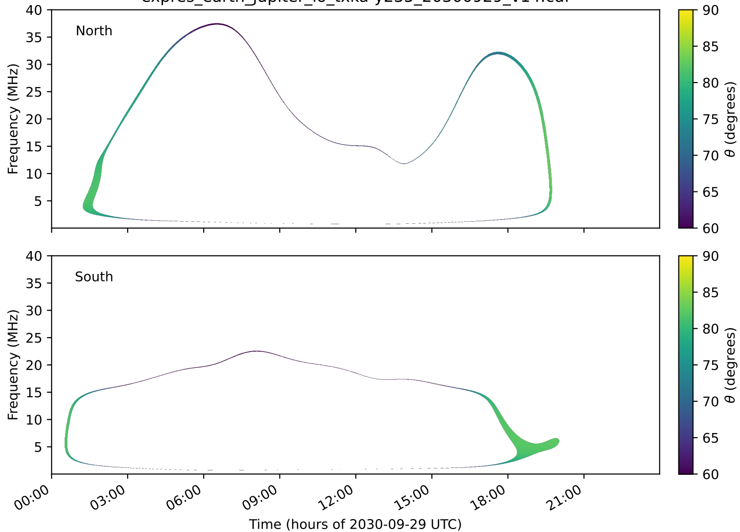
expres_earth_jupiter_io_txka-y235_20300929_v14.cdf
