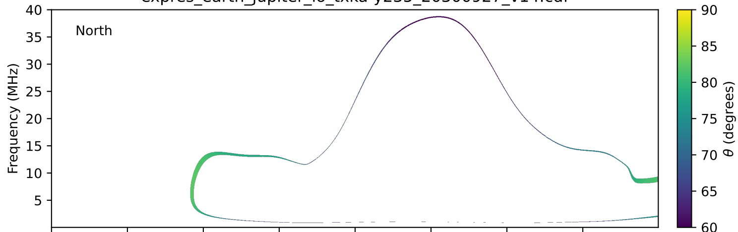
expres_earth_jupiter_io_txka-y235_20300927_v14.cdf
