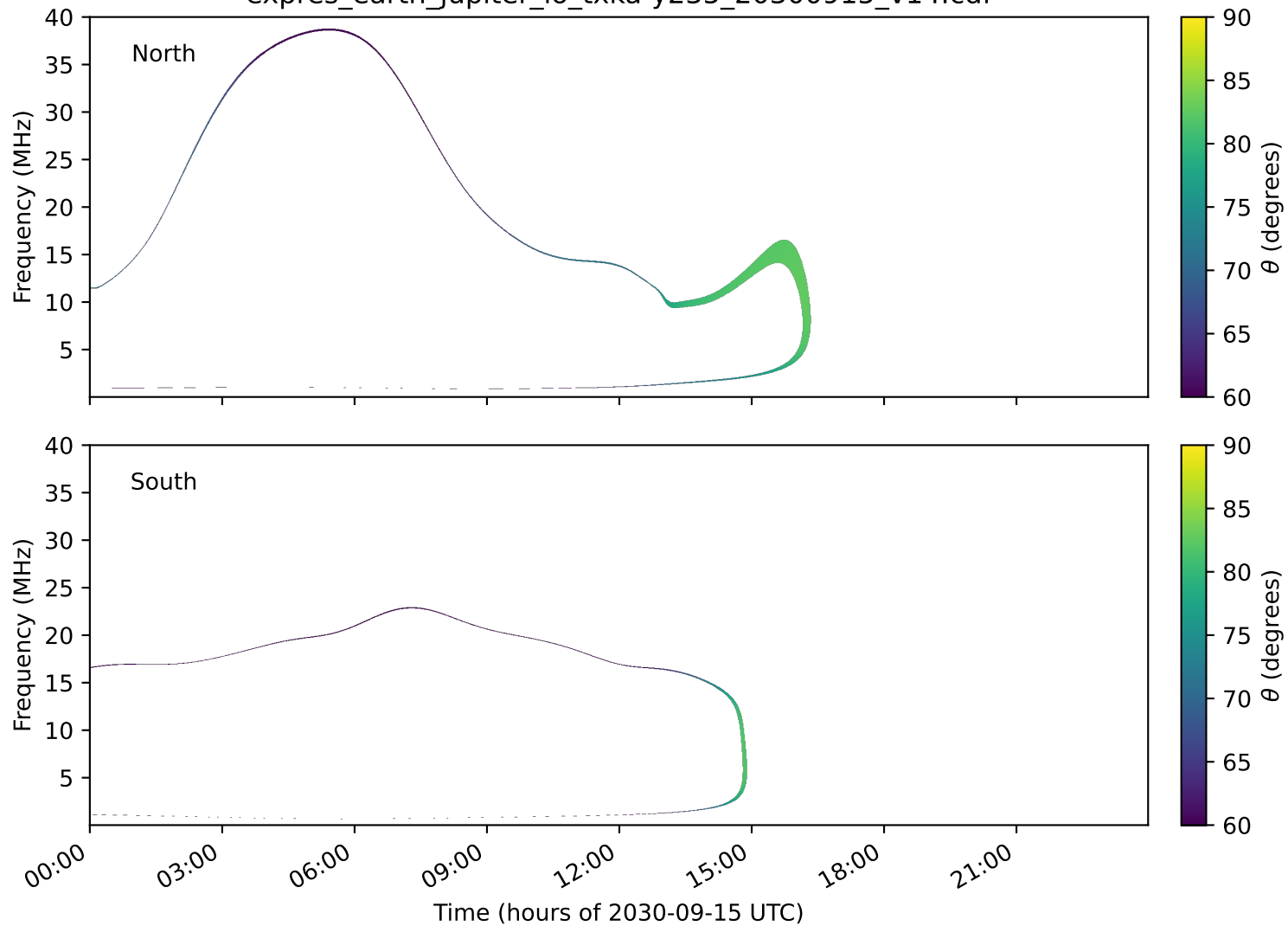
expres_earth_jupiter_io_txka-y235_20300915_v14.cdf
