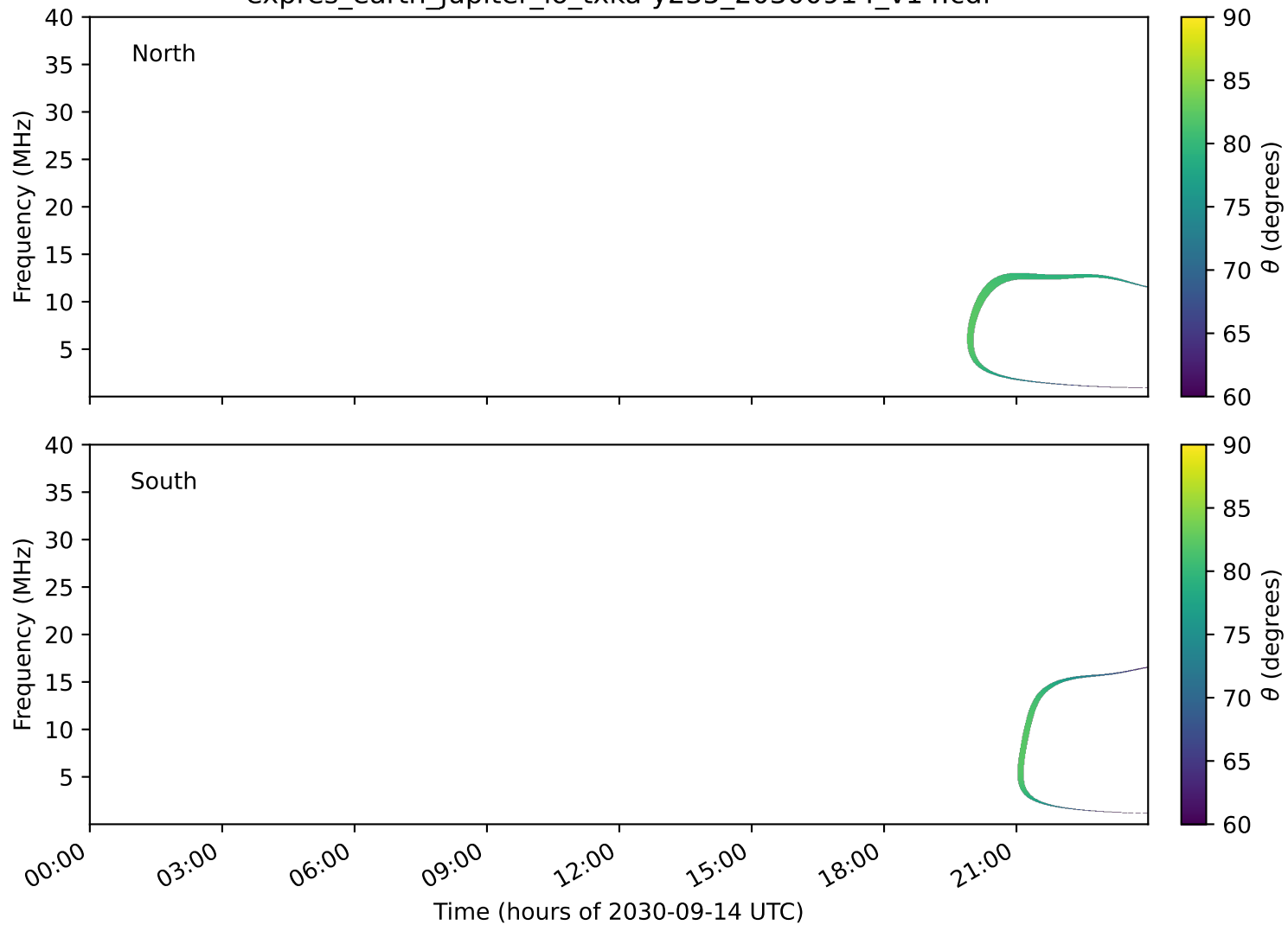
expres_earth_jupiter_io_txka-y235_20300914_v14.cdf
