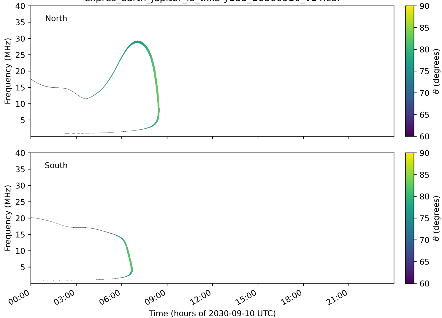
expres_earth_jupiter_io_txka-y235_20300910_v14.cdf
