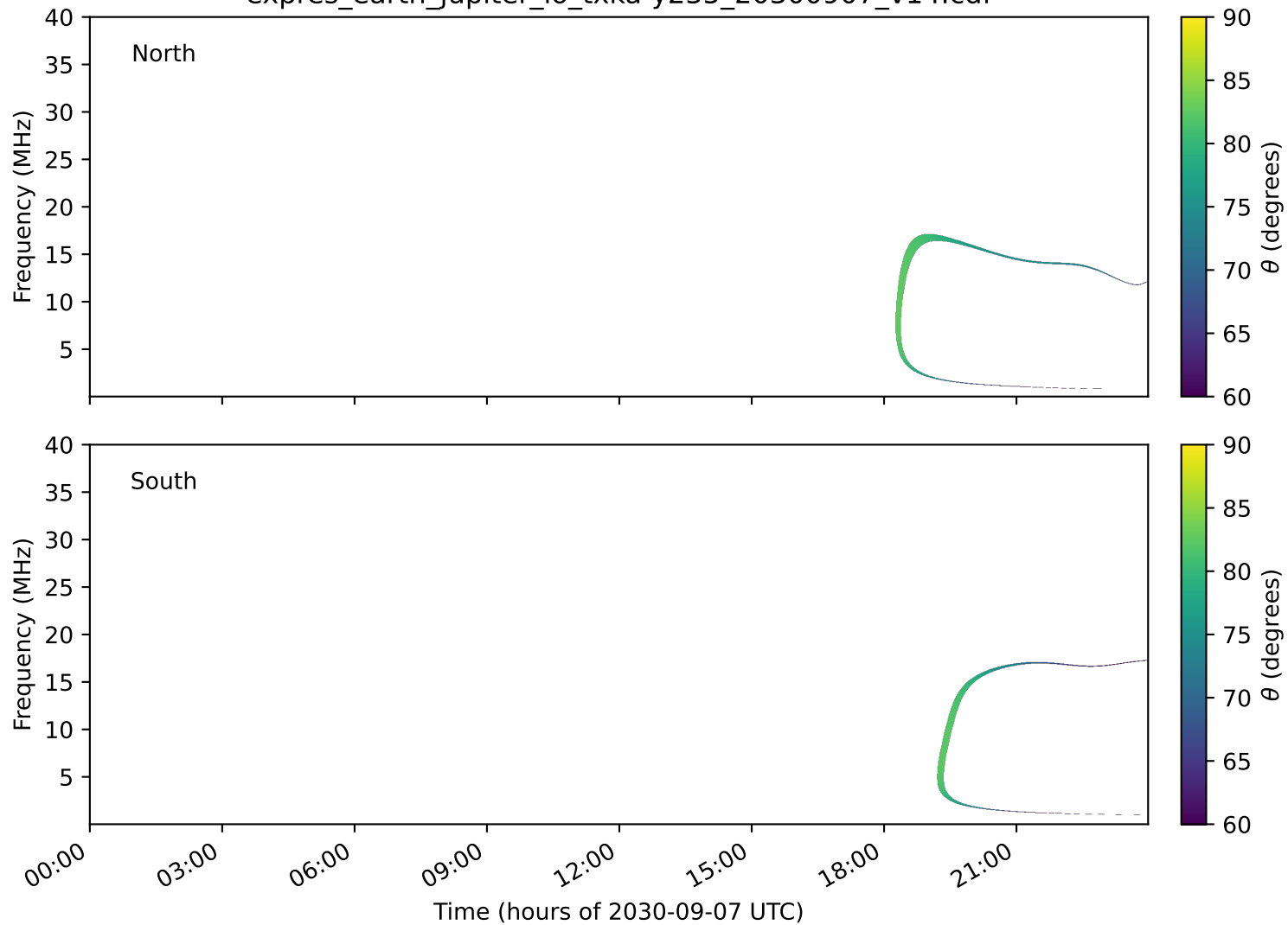
expres_earth_jupiter_io_txka-y235_20300907_v14.cdf
